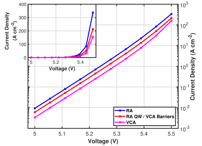
FIG. 2. (a) Current-voltage curves, on a log-scale, for an \text{Al}_{0.7}\text{Ga}_{0.3}\text{N}/\text{Al}_{0.8}\text{Ga}_{0.2}\text{N} quantum well embedded in a p - n junction. The data are shown for simulations that (i) account for random alloy (RA) fluctuations in the well and barriers (blue), (ii) account for RA fluctuations in the well but treat the barrier in a virtual crystal approximation (VCA) (red), and (iii) use a VCA in the entire p - i - n structure (pink). The inset shows the I-V curves on a linear scale.
