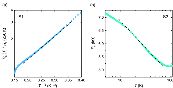
FIG. 3. (a) Normalized sheet resistance (on a log scale) versus T^{-1/3} for pristine S1. The dashed line is the linear fitting result. (b) Sheet resistance R_s as a function of temperature T (on a log scale) for pristine S2. The linear regime (dashed line) shows that the resistance varies as \ln(1/T) .
