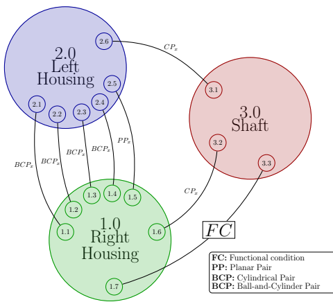
Figure 3: Contact graph of the pump
