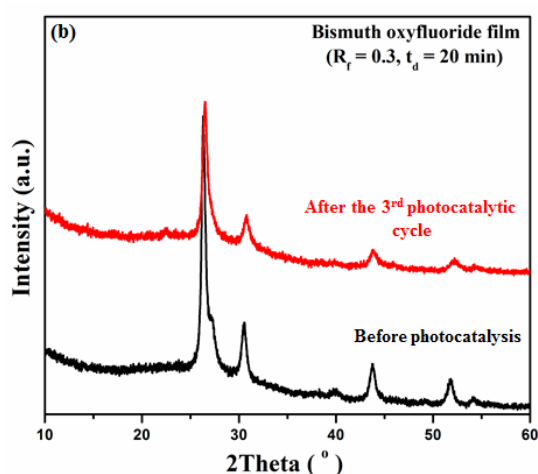
Figure S2: XRD pattern for the film deposited for R_f = 0.3 for 20 min, before and after 3 cycles of 2 hours of photodegradation experiment.
