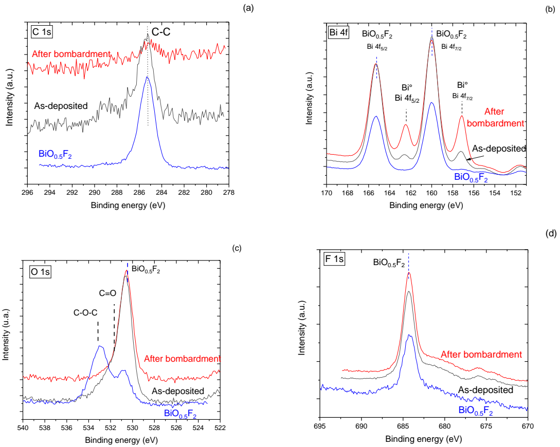
Figure 8: XPS spectra obtained for (a) C 1s, (b) Bi 4f, (c) O 1s and (d) F 1s for film deposited at R_f = 0.3 for 20 min, before and after \text{Ar}^+ bombardment and for \text{BiO}_{0.5}\text{F}_2 powder.
