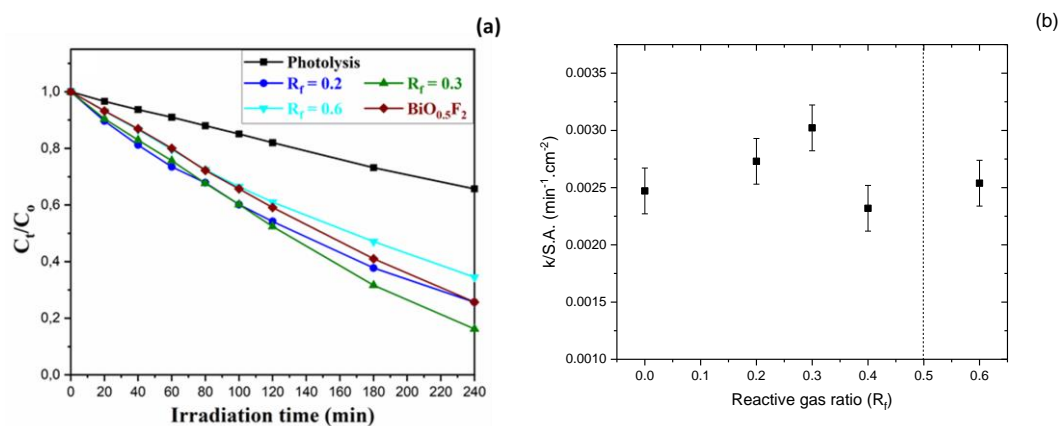
Figure 4: (a) Degradation of MO ( C_t/C_0 ) as a function of the irradiation time in the presence of films ( R_f = 0.2 , 0.3 , and 0.6 ) and \text{BiO}_{0.5}\text{F}_2 powder, and (b) the reaction rate to surface area, k/S.A. , as a function of R_f .
