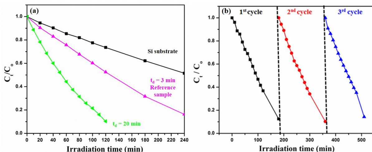
Figure 10: (a) Degradation of MO ( C_t/C_0 ) as a function of the irradiation time in the presence of films obtained at R_f = 0.3 for 3 and 20 min of deposition times and (b) cycling curves of photocatalytic degradation for the one deposited during 20 min.
