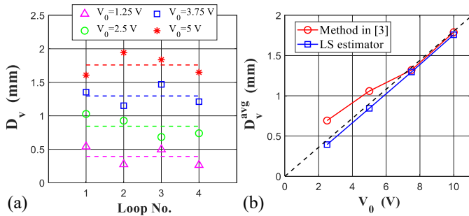
Fig. 4. (a) Estimated vibration amplitude for four voltage levels feeded to speaker using loop No.1 to 4. Average value at each level is shown in dashed line. (b) Averaged estimated amplitude as a function of voltage. Straight line is depicted in black dashed line for comparison.
