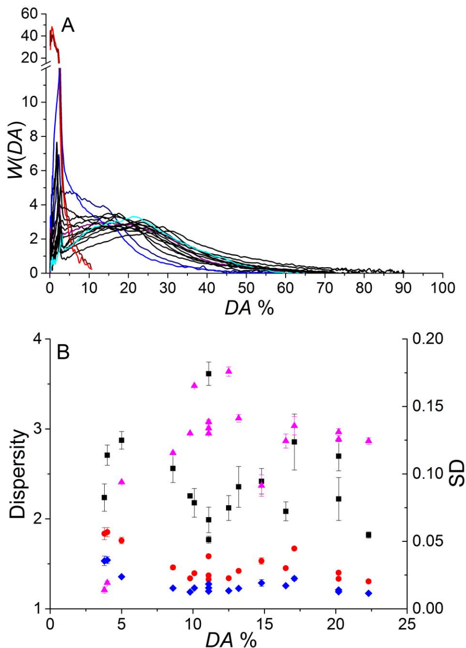
Figure 9. A. Composition distributions and B. Dispersity of composition distributions as D(W(DA),1,0) (black squares), D(W(DA),2,0) (red circles), D(W(DA),3,0) (blue diamonds) and standard deviation (pink triangles) for chitosan samples separated in LiPB100 and treated with the 2nd iteration. See supporting information equation S1 to S8 for dispersity calculations [27].
