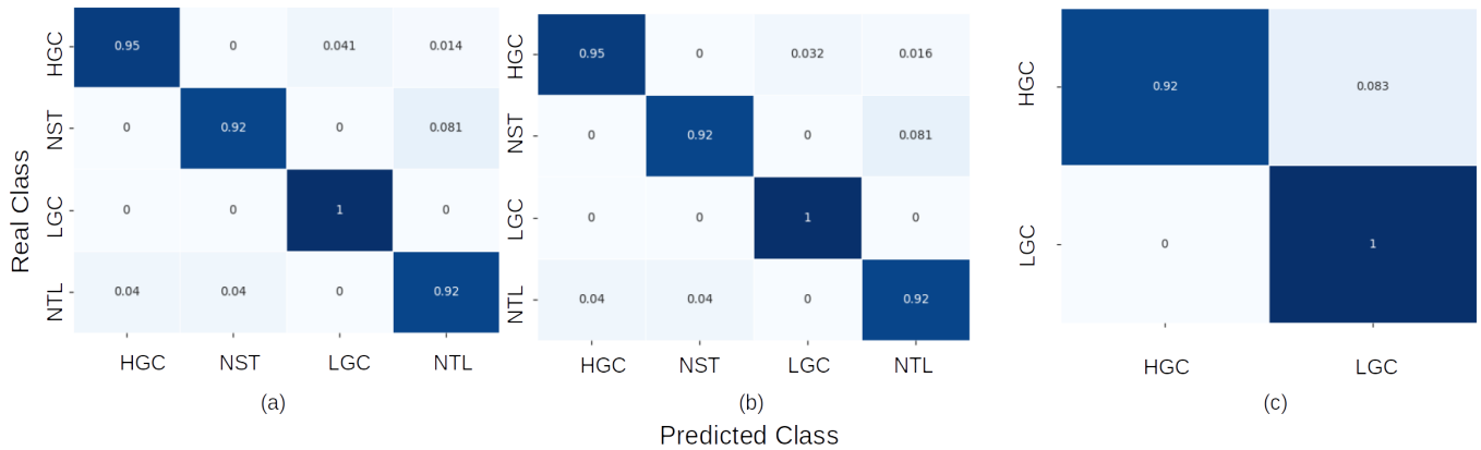
Fig. 6: Confusion matrices of the best model obtained. a) Analysis on the complete test data (WLI + NBI). b) Analysis only on the WLI test data. c) Analysis on the NBI data. It is important to notice that due to the scarcity of annotated NBI data, the NBI test dataset was composed only of HGC and LHC images.
