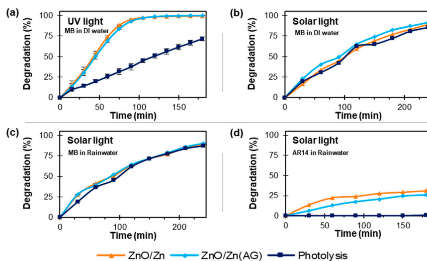
Figure 3. MB photodegradation with and without ZnO NSs under (a) UV light source ( \sim 365 nm, 35 mW/cm ^2 ) in DI Water, (b) natural solar light (April/May, France, I_{UV} = 2.3 mW/cm ^2 ) in DI Water, and (c) natural solar light (April/May, France, I_{UV} = 2.3 mW/cm ^2 ) in rainwater; (d) AR14 photodegradation with and without ZnO NSs under natural solar light (April/May, France, I_{UV} = 2.9 mW/cm ^2 ) in rainwater.
