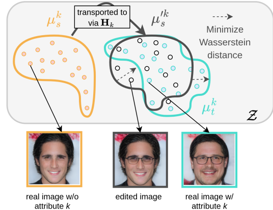
Fig. 1: Method overview. For each semantic attribute ( e.g. “Glasses”) we learn a mapping H_k that moves the distribution of latent codes lacking the attribute to the distribution of codes having that attribute. We enforce that each latent code is moved near a point that shares similar semantics, thus only changing that attribute. For identity preservation, the resulting distribution does not entirely match the target distribution.
