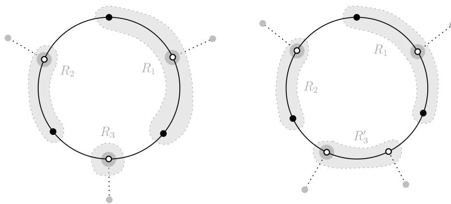
Figure 5: A cycle reduction. On the left, an even cycle with potential \Phi_I(R_1, R_2, R_3) = -2 + 0 + 2 = 0 and on the right an odd cycle with potential -1 . Vertices surrounded by a grey disk are the ones picked by the algorithm and dotted edges are debt edges.
