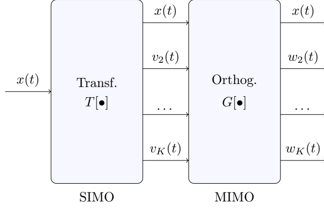
Figure 3: OSG block diagram of our proposed method. In the SIMO sub-part, the K output signals are obtained from a transformation T[\bullet] defined in equations (1, 6, 10, 14, 17). The K mutually orthogonal signals are obtained with the Gram-Schmidt procedure (a kind of transformation G[\bullet] ) in the MIMO sub-part. As for OSG represented in figure (2), the following relations must be verified: v_1(t) = w_1(t) = x(t) .
