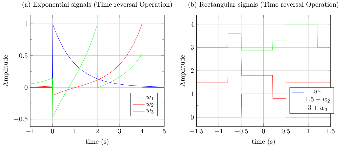
Figure 9: a) Orthogonal atoms obtained for w_1(t) = e^{-at}u(t) with a = 1 , \tau_1 = 4 , \tau_2 = 2 , \gamma_{21} = -0.147 , \gamma_{31} = -0.619 and \gamma_{32} = 0.533 . b) Orthogonal atoms obtained for w_1(t) = \text{Rect}_T(t) with T = 1 s, \tau_1 = 0.2 , \tau_2 = -0.4 , \gamma_{21} = -0.702 , \gamma_{31} = -0.714 and \gamma_{32} = 0.590 .
