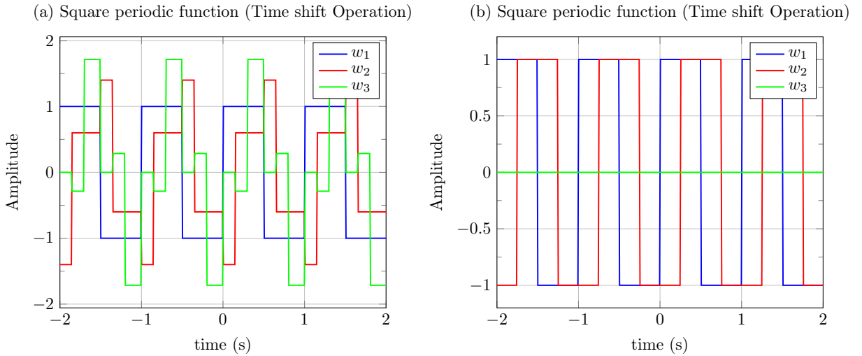
Figure 6: (a) Innovative orthogonal atoms obtained with time shifts \tau_1 = -0.15 s, \tau_2 = -0.15 s, \gamma_{21} = -0.400 , \gamma_{31} = 0.857 , \gamma_{32} = -0.143 , the first atom being defined by v_1(t) = \text{sign}(\sin(\omega t)) with T = 1 s. (b) Orthogonal atoms obtained with time shifts \tau_1 = -0.25 s, \tau_2 = -0.25 s, \gamma_{21} = 0 , \gamma_{31} = 1 , \gamma_{32} = 0 , the first atom being defined by v_1(t) = \text{sign}(\sin(\omega t)) with T = 1 s.
