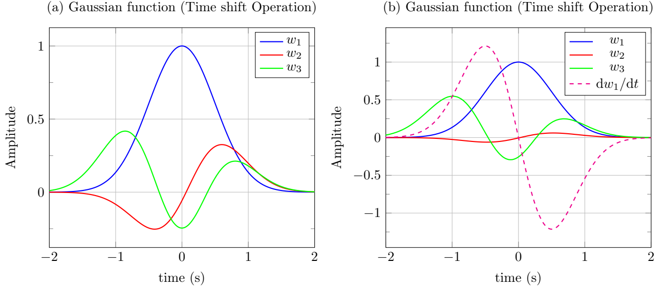
Figure 5: (a) Orthogonal Gaussian atoms obtained with time shifts \tau_1 = 1/4 s and \tau_2 = -3/4 s, and with a = 2 , \rho_{21} = \rho(1/4) = 0.94 , \rho_{31} = \rho(1/4 + 3/4) = 0.78 , \rho(3/4) = 0.57 , \rho_{32} = -1.38 , \gamma_{21} = -0.94 , \gamma_{31} = -2.07 and \gamma_{32} = 1.38 ; the first atom being defined by v_1(t) = e^{-at^2} . (b) Innovative orthogonal Gaussian atoms obtained with time shifts \tau_1 = 0.05 s, \tau_2 = -3/4 s, a = 2 , \rho_{21} = 1.00 , \rho_{31} = 0.61 , \rho(3/4) = 0.57 , \rho_{32} = -8.28 , \gamma_{21} = -1.00 , \gamma_{31} = -8.88 and \gamma_{32} = 8.29 , the first atom being defined by v_1(t) = e^{-at^2} . The derivative of the Gaussian function is reported in dashed line with \tau = -1/4 meaning that the derivative is (-4) times higher than w_2(t) .
