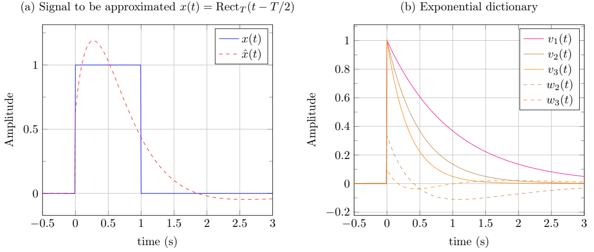
Figure A.12: a) Rectangular signal x(t) to be approximated and its approximation \hat{x}(t) (in dashed line). b) Exponential dictionary with v_1(t), v_2(t), v_3(t) and its orthogonal basis w_1(t) = v_1(t), w_2(t), w_3(t) (dashed line).
