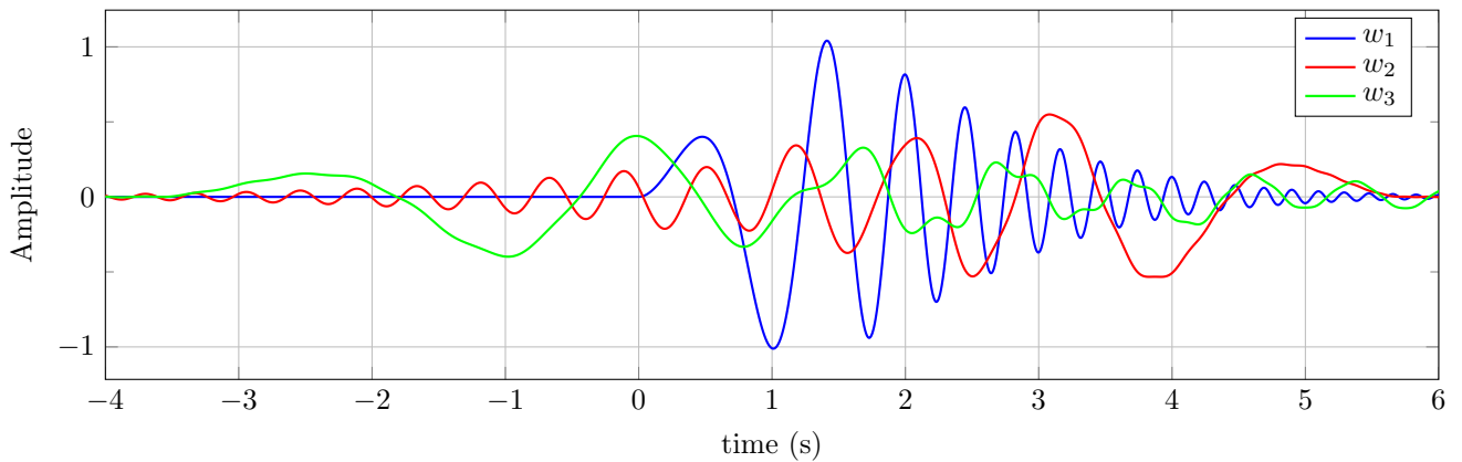
Figure 11: Orthogonal atoms obtained numerically from the transformation T_k[v_1] = \alpha_k + \beta_k v_1((-1)^k \beta_k t + \tau_k) and for the generator signal v_1(t) = t^2 e^{-at} \cos(2\pi f t^2) with K = 3 . The sampling frequency is of F_s = 1000 Hz.
