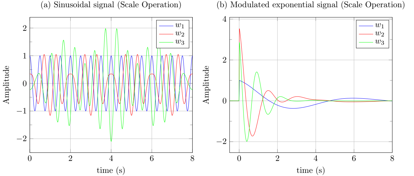
Figure 8: a) Orthogonal atoms obtained scale change with \beta_1 = 3/4 and \beta_2 = 5/4 , \gamma_{21} = -0.409 , \gamma_{31} = -0.543 , \gamma_{32} = -0.830 ; the first atom being defined by v_1(t) = \cos(2\pi ft) for f = 4 Hz. b) Orthogonal atoms obtained with w_1(t) = \cos(2\pi t/T)e^{-at}u(t) with \beta_2 = 4 , \beta_3 = 3/2 , a = 1/3 , \omega = 3a , \gamma_{31} = -0.058 , \gamma_{32} = -0.746 and \gamma_{21} = -0.403 .
