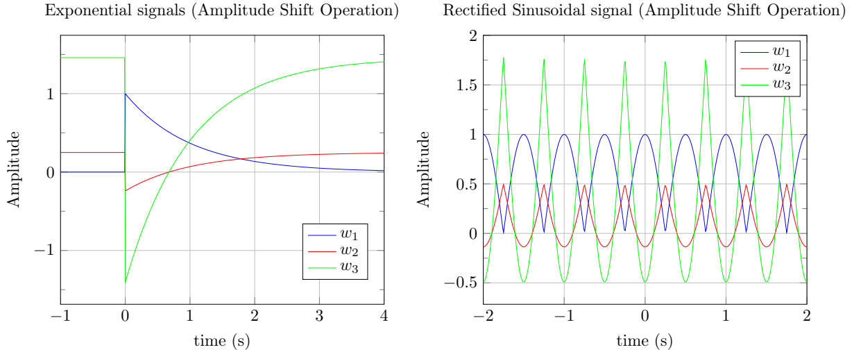
Figure 10: (a) Orthogonal atoms obtained by amplitude shift, \alpha_1 = 1/4 , \alpha_2 = 1/4 , the first atom being defined by w_1(t) = e^{-at}u(t) , with a = 1 , \gamma_{21} = -1.491 , \gamma_{31} = -7.701 and \gamma_{32} = 3.835 . (b) Orthogonal atoms obtained by amplitude shift \alpha_1 = 1/2 , \alpha_3 = 3/4 . The first atom being defined by w_1(t) = |\cos(2\pi ft)| , with f = 1 Hz, \gamma_{21} = -1.636 , \gamma_{31} = -5.379 and \gamma_{32} = 2.093 .
