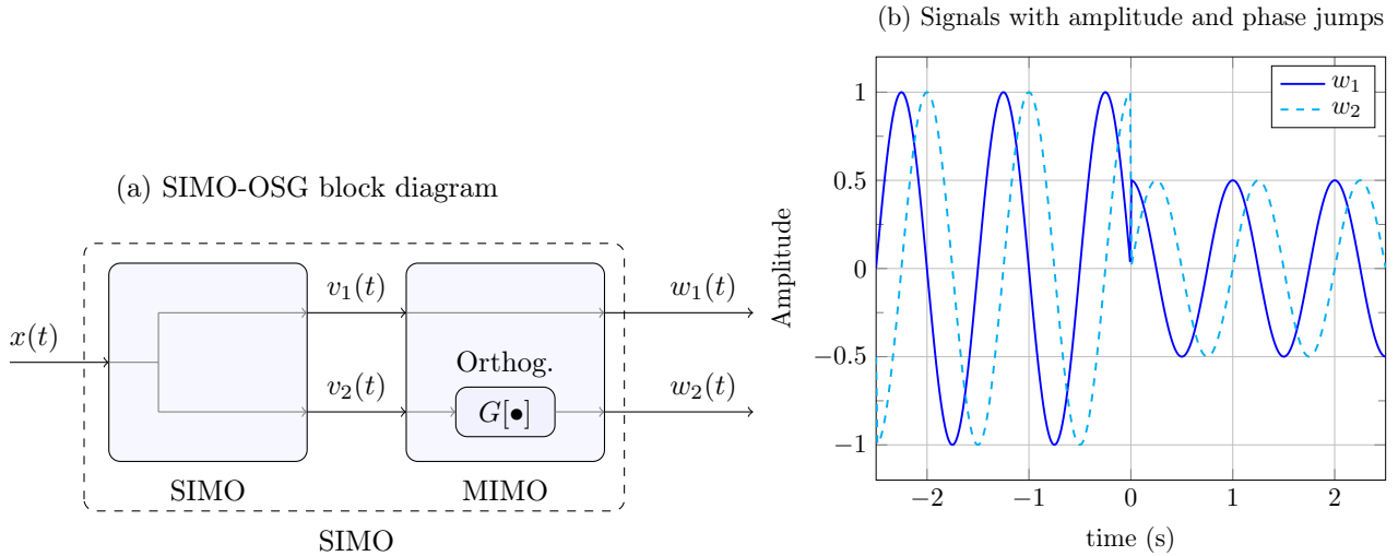
Figure 2: a) Common partial block diagram of a SIMO-OSG in electrical engineering. As in figure (1), the SIMO system can be separated in two sub-parts: another SIMO system followed by a MIMO system with v_1(t) = w_1(t) = x(t) , v_2(t) = x(t) and with orthogonalized signal w_2(t) being obtained through a transformation G[\bullet] as derivative, Hilbert transform, ... b) Periodic signal w_1 = x(t) undergoing a phase and an amplitude jumps at t = 0 and its orthogonalized version w_2(t) obtained by applying the method of section 2.1.
