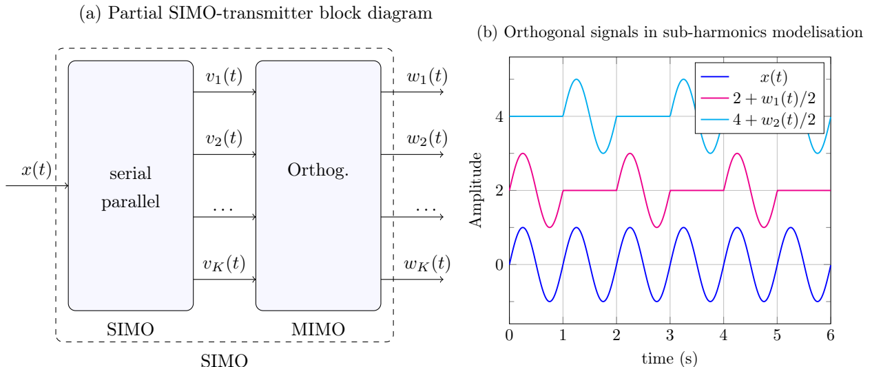
Figure 1: a) Partial block diagram of a transmission/modelisation system as a Single Input Multiple Output (SIMO) system. This SIMO system can be separated in a serial-parallel converter (another SIMO system) followed by a MIMO (Multiple Input and Multiple Output) system composed of K mutually orthogonal signals. Usually, the orthogonalization function is merged with the serial/parallel function. b) Orthogonal signals used in non linear systems modelisation in control engineering with sub-harmonics [1, 25], with x(t) = w_1(t) + w_2(t) .
