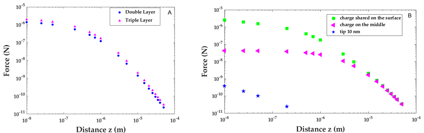
Figure 3. (A) Modeling of the interaction between a surface covered by dipoles and a charged sphere of 10 μm diameter by considering the simplified double layer (blue sphere) or triple layer model (pink triangles); and (B) modeling of the impact of the charge's discretization on sphere surface. Repulsive force obtained between a dipole surface and a 10 μm charged sphere with the charge fairly shared on the surface (green squares), centered at the middle of the sphere as a point charge: the same charge as previous, but located in the sphere center (pink triangles) or 10 nm charged tip (blue stars).
