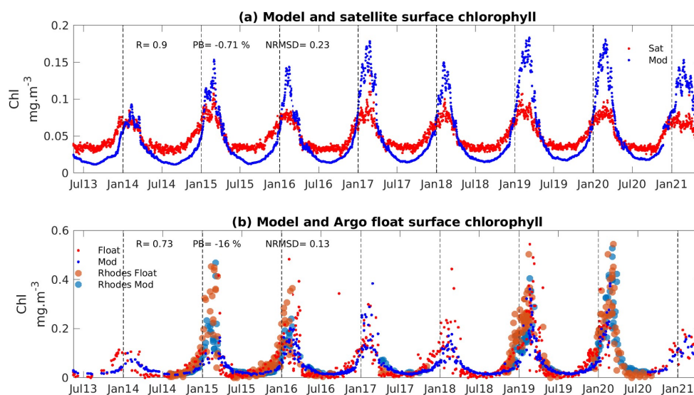
Figure 2: Time series of (a) modeled (in blue) and satellite (in red) surface chlorophyll-a concentration ( \text{mg m}^{-3} ) averaged over the Levantine Basin, and of (b) modeled (in blue) and BGC-Argo float (in red) surface chlorophyll-a concentration ( \text{mg m}^{-3} ) in the Levantine Basin; light-colored dots represent data located in the Rhodes Gyre. Coefficient correlation (R), percent bias (PB) and Normalized Root Mean Square Deviation (NRMSD) between model outputs and observations are indicated in (a) and (b).
