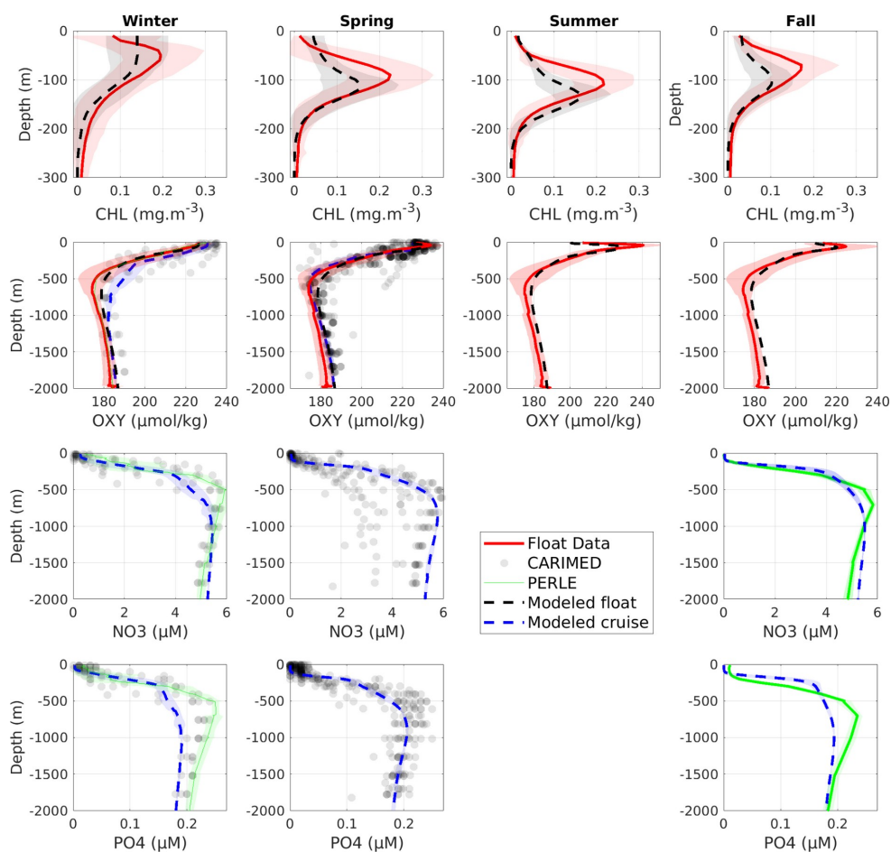
Figure 3: Comparison over the Levantine Sea between observed (gray points for CARIMED, green lines for PERLE1 and PERLE2, red line for BGC-Argo float data) and modeled (blue and black lines) profiles of chlorophyll ( \text{mg Chl m}^{-3} ), dissolved oxygen ( \mu\text{mol kg}^{-1} ), nitrate ( \mu\text{M} ) and phosphate ( \mu\text{M} ) concentrations, averaged by season (winter: 21 December to 20 March, spring: 21 March to 20 June, summer: 21 June to 20 September, fall: 21 September to 20 December). Shaded areas represent standard deviation.
