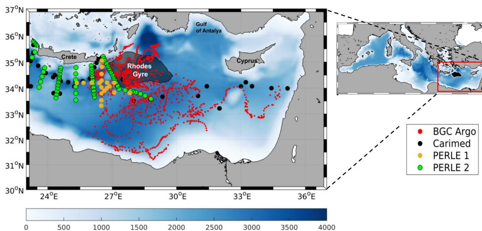
Figure 1: Model domain (right) and bathymetry (m) in the Mediterranean Sea and Levantine Basin. Red, black, yellow and green dots indicate positions of BGC-Argo floats, CARIMED, PERLE 1 and PERLE 2 cruise data, respectively, from 2013 to 2020. The black patch represents the Rhodes Gyre.
