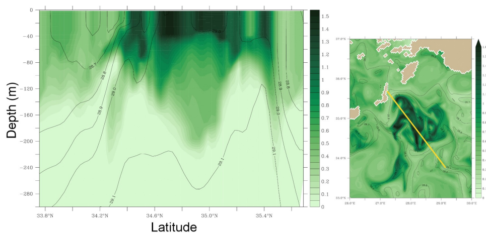
1315 Figure 12: Vertical section of phytoplankton concentration (expressed in mmol C m -3 ) across the Rhodes Gyre on March 27, 2015. The potential density anomaly (kg m -3 ) is overlaid with contours. The position of the section is indicated on the map of surface phytoplankton (right panel).
