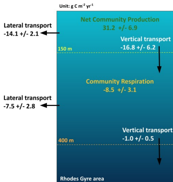
1300 Figure 9: Annual organic carbon budget (g C m -2 yr -1 ) in the surface and intermediate layers of the Rhodes Gyre for the seven year period 2013-2020.
