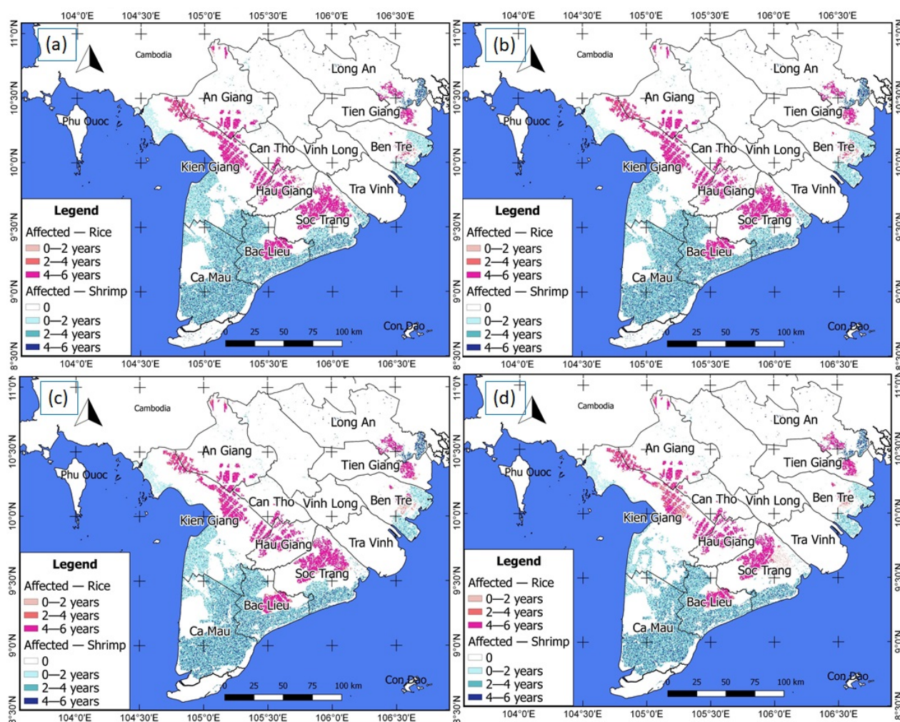
Figure 6. Vulnerability maps for rice and shrimp until 2050. (a) Experiment 1: Baseline 1; (b) Experiment 2: Baseline 2, subsidence impact; (c) Experiment 3: Reaction to subsidence of 0.1 m; (d) Experiment 4: Reaction to subsidence of 0.1 m along with an adaptation mechanism.
