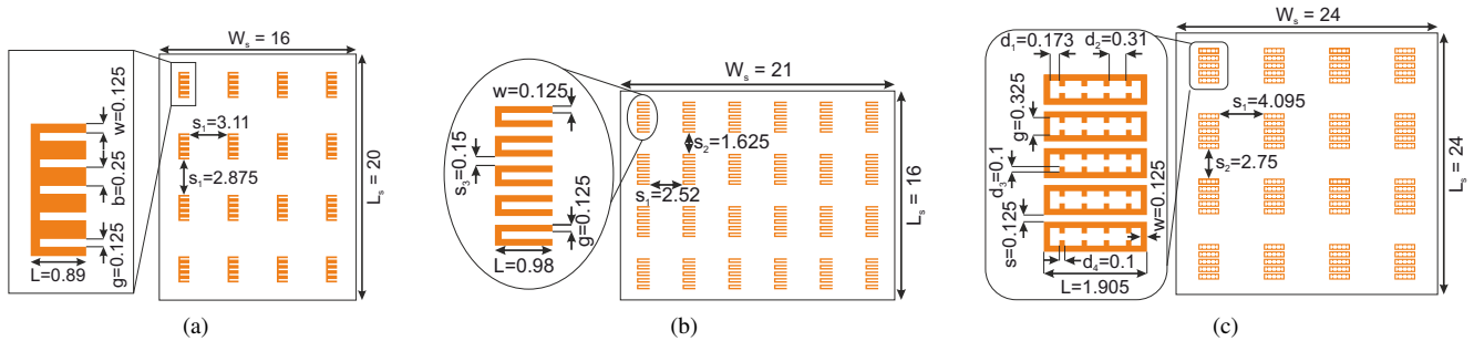
Fig. 2: Design dimensions for the tags without a ground plane. (a) E-shape, (b) C-shape and (c) L-shape. All dimensions are in millimeters.
