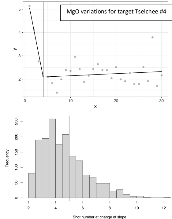
Figure 3: a. Slope change detection for MgO for target Tselchee #4 b. Histogram of slope change detection indicating that most of the changes occur at or below 5 shots.
