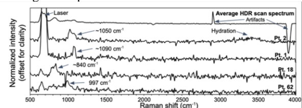
Figure 6: SHERLOC Raman spectra of Dourbes showing mineral peaks and possible hydration (labeled) [8].
