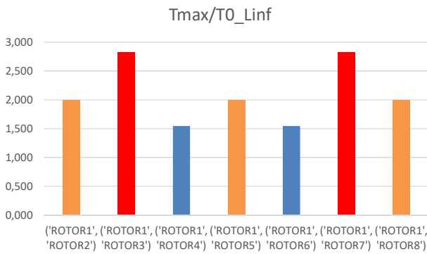
Figure 6: Maximum thrust ratios depending on which couple of rotors is in failure for the Octo "PNPN"
