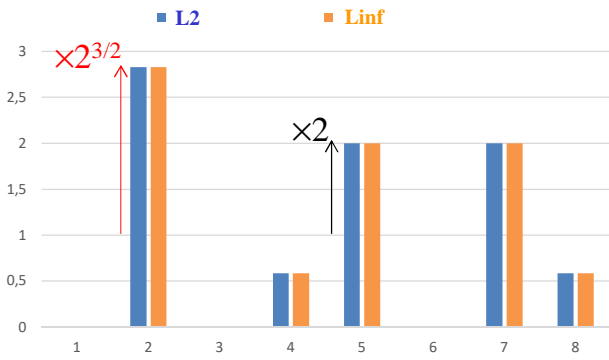
Figure 4: Normalized thrusts redistribution for rotors 1 & 3 in failure – Worst case for the Octo+ of Figure 2
