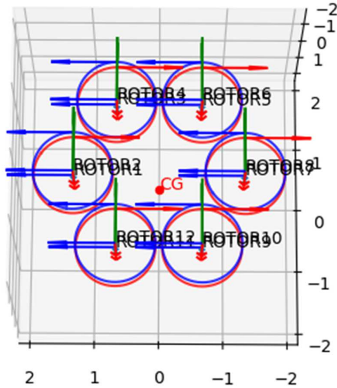
Figure 15: configuration with 12 coaxial rotors.
