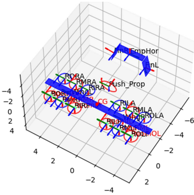
Figure 20: fully symmetrical configuration with diametrically opposite rotors turning in opposite direction
