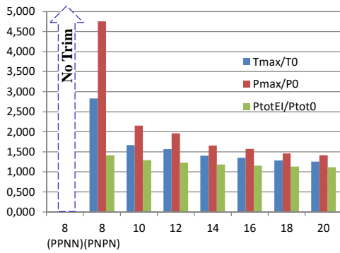
Figure 10: maximum ratios of thrust, power and total power for the worst double rotor failure for different numbers of rotors
