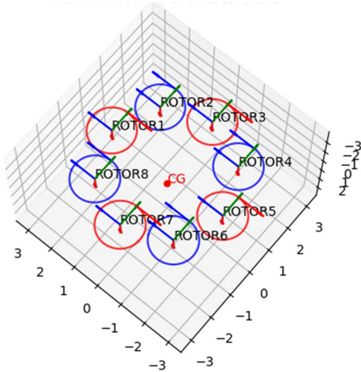
Figure 2: Octo+ configuration (“PNPN”)
