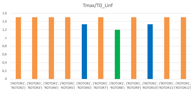
Figure 16: \frac{T_{max}}{T_0} for the 11 cases of double failures with the 12 coaxial rotors configuration.
