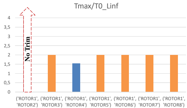
Figure 8: Maximum thrust ratios depending on which couple of rotors is in failure for the Octo "PPNN"
