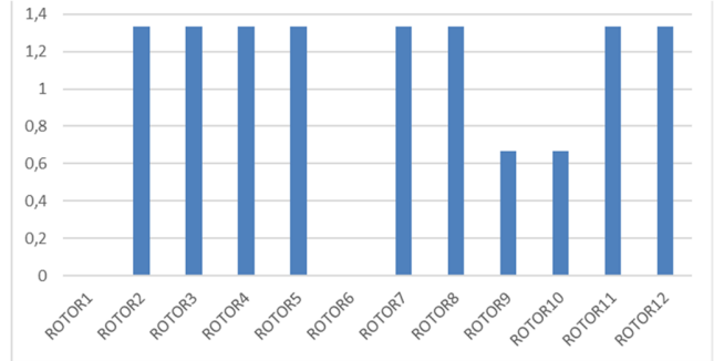
Figure 17: Optimal- L_\infty thrust redistribution for the nearly symmetrical cases of double failure (e.g. 1&6).
