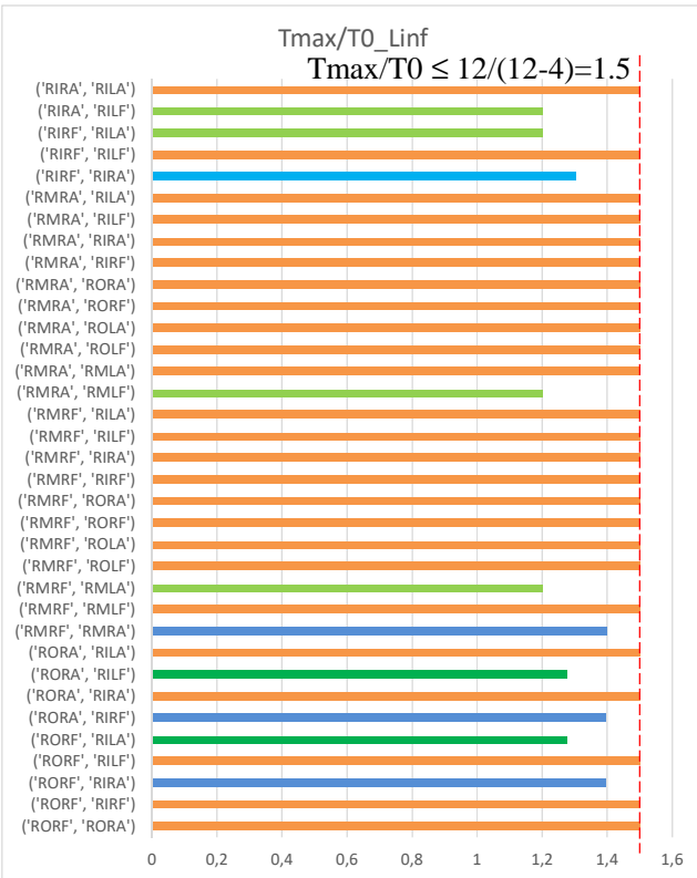
Figure 21: ratios of maximum thrust augmentation for coping with a double rotor failure (half cases presented taking into account the right/left symmetry, case of configuration on Figure 20)
