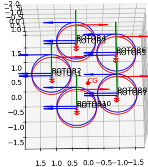
Figure 13: configuration with 10 coaxial rotors.
