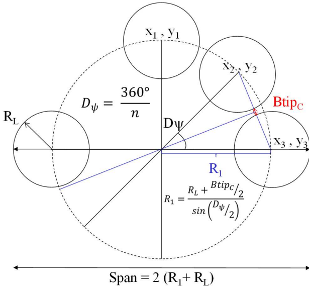
Figure 9: circular axi-symmetrical configurations for any number of n lifting rotors
