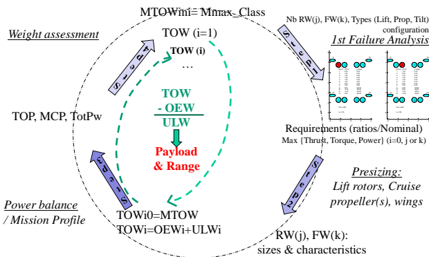
Figure 1: First Presizing Loop, convergence on DGW
