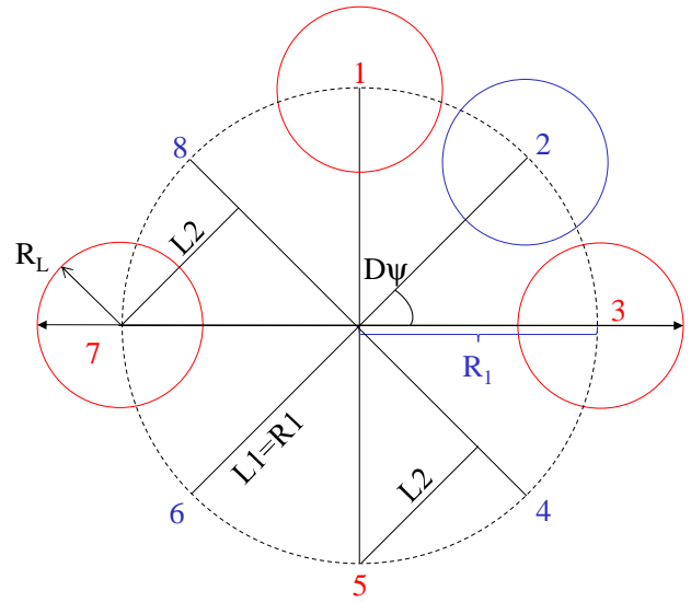
Figure 5: Geometrical description of the Octo case.
