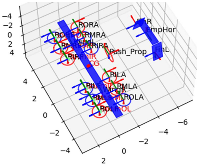
Figure 18: Simplified Cora configuration with original directions of rotation
