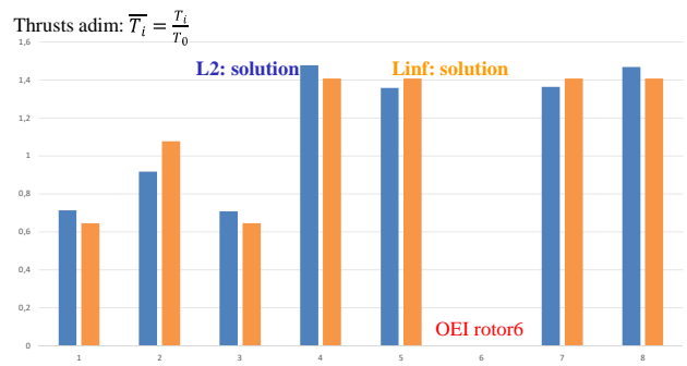
Figure 3: Example of two optimal L_2 or L_\infty thrusts redistributions for a failure on rotor 6 in the “Octo+” case.
