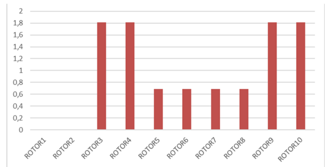
Figure 14: thrusts optimal redistribution on the 10 coaxial rotors configuration for coping with rotors 1&2 failures
