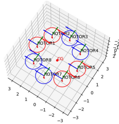
Figure 7: Octo+ configuration ("PPNN")
