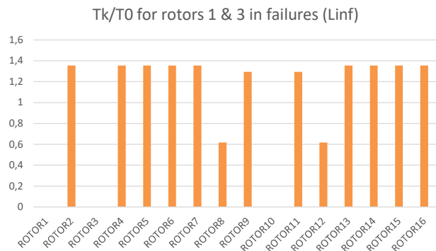
Figure 11: Thrusts redistribution for the case with 16 rotors and rotors 1 & 3 in failure
