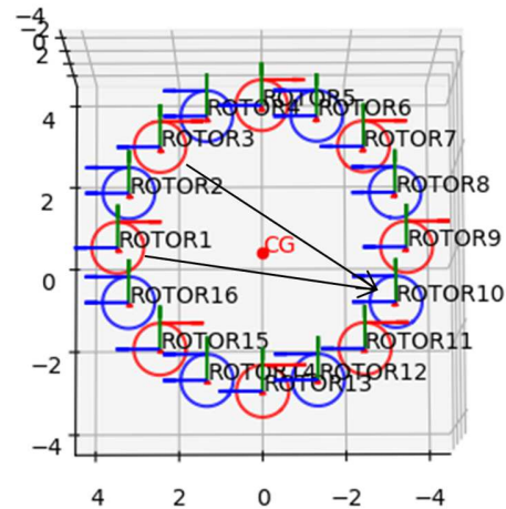
Figure 12: Scheme of the 16 rotors with rotors 1 & 3 in failures
