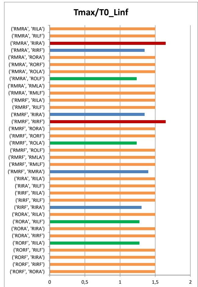
Figure 19: ratios of maximum thrust augmentation for coping with a double rotor failure (half cases presented taking into account the right/left symmetry, case of configuration on Figure 18)
