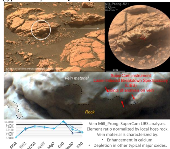
Fig. 3: Composition of a light-toned vein as analyzed with the SuperCam instrument's LIBS technique. Mastcam-Z image ID: ZLF_0510_0712218603_973RAD_N0261222CAM08533_1100LMJ01.
