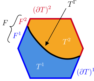
Figure 2: Decomposition of a cut cell T \in \mathcal{T}^\Gamma and of its boundary \partial T .
