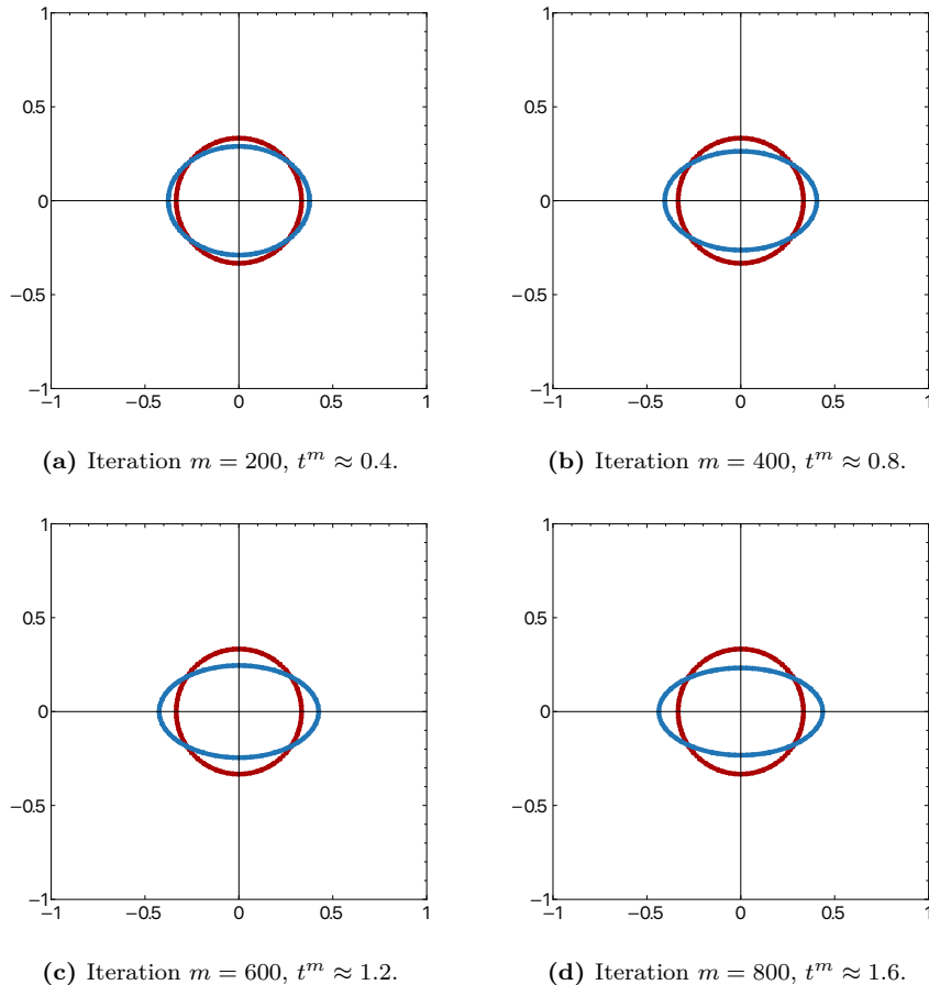
Figure 14: Second verification test case: Ca = 0.27 (i.e., \varepsilon = 0.4 , \gamma = 1 , \mu_2 = 1 , R_* = 1/3 ). In each panel, the red bullets represent the initial interface, and the blue ones the interface at iteration m of the fixed-point procedure. The HHO polynomial order is k = 1 , and we employ q = 2 for the level-set approximation. The mesh is composed of 64 \times 64 square cells. The interface discretization parameters are (l = 2, n = 0) .
