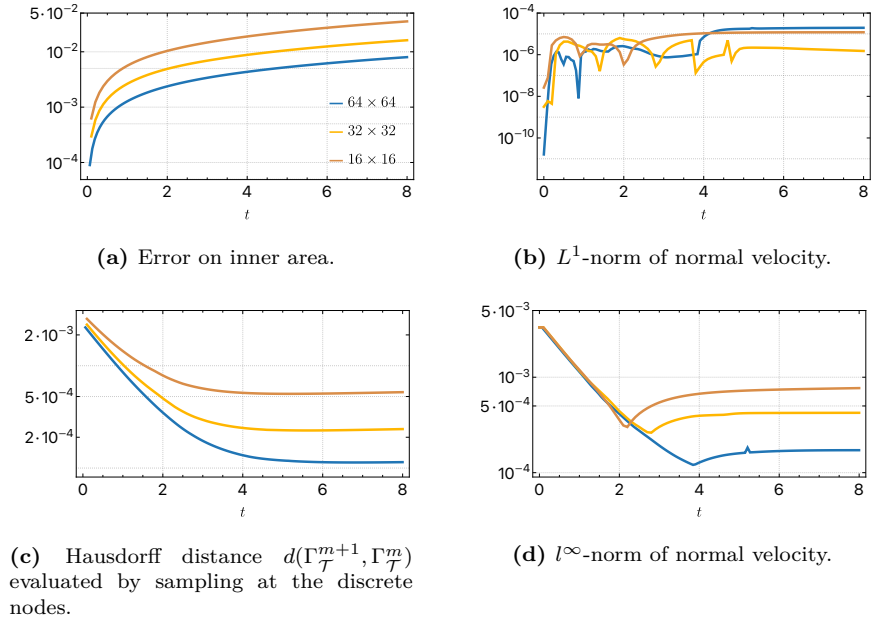
Figure 16: Second verification test case: error indicators for Ca = 0.007 (i.e., \varepsilon = 0.01 , \gamma = 1 , \mu_2 = 1 , R_* = 1/3 ) for various levels of mesh refinement. The HHO polynomial order is k = 1 , and we employ q = 2 for the level-set approximation. The meshes are composed of 16 \times 16 (brown line), 32 \times 32 (yellow line) and 64 \times 64 (blue line) square cells. The interface discretization parameters are (l = 2, n = 0) . The number of fixed-point iterations is 21, 34, and 66 for 16 \times 16 , 32 \times 32 , and 64 \times 64 square cells, respectively.
