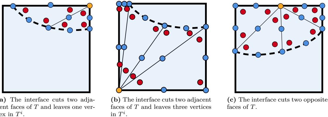
Figure 5: Example of cut cells T \in \mathcal{T}^\Gamma and of their decomposition into curved subtriangles. The subtriangulation is performed by connecting the interface points \{\mathbf{x}_m^{T,j}\}_{m \in \{0:2\}, j \in \{1:2^n\}} to a specific point (orange bullet, a vertex or an edge midpoint according to the cut configuration). The interface discretization parameters are (l = 2, n = 1) . The blue bullets, plus the orange bullet, are the physical points used for defining the mapping from the reference triangle into the physical one (quadratic mapping in the present example). Moreover, the red bullets represent the mapped integration Dunavant points for the second-order quadrature.
