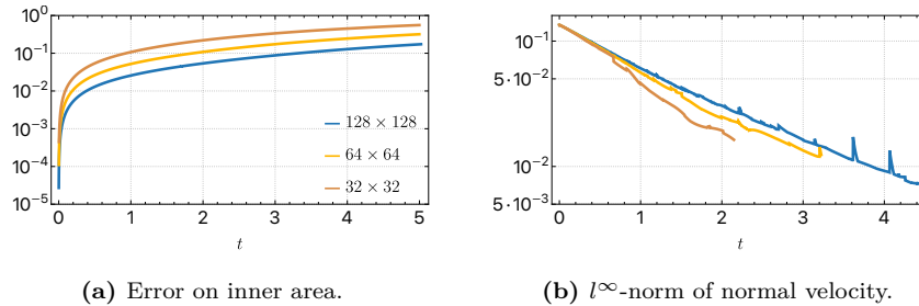
Figure 19: Error indicators for Ca = 0.27 (i.e., \varepsilon = 0.26 , \gamma = 1 , \mu_2 = 1 , R_* = 1/3 ) for various levels of mesh refinement. The HHO polynomial order is k = 1 , and we employ q = 2 for the level-set approximation. The meshes are composed of 32 \times 32 (brown line), 64 \times 64 (yellow line) and 128 \times 128 (blue line) square cells. The interface discretization parameters are (l = 2, n = 0) . The number of fixed-point iterations is 21, 2400, and 5100 for 32 \times 32 , 64 \times 64 , and 128 \times 128 square cells, respectively.
