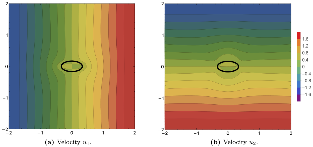
Figure 9: Shear-surface tension equilibrium with elliptic interface: isovalues of the velocity components \mathbf{u} = (u_1, u_2) for D = 1/3 , \mu_1 = \mu_2 = 1 , Ca = 0.28 (i.e., \varepsilon = 0.59 , \gamma = 1 , R_1 = 1/6 and R_2 = 1/3 ) in the domain \Omega = (-2, 2)^2 discretized by a mesh composed of 128 \times 128 square cells. We employ the unfitted HHO discretization with polynomial order k = 1 .
