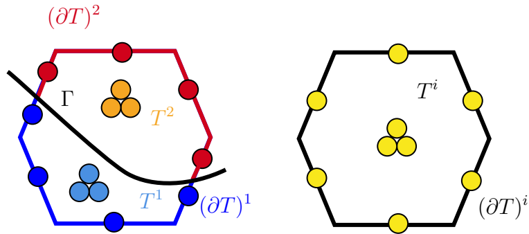
Figure 3: Discrete velocity unknowns ( k=0 ) for a cut (left) and uncut (right) cell of hexagonal shape. Notice the doubling of the cell unknowns in the cut cell and of the face unknowns on the cut faces. Conventionally, each bullet represents one \mathbb{R}^2 -valued degree of freedom.
