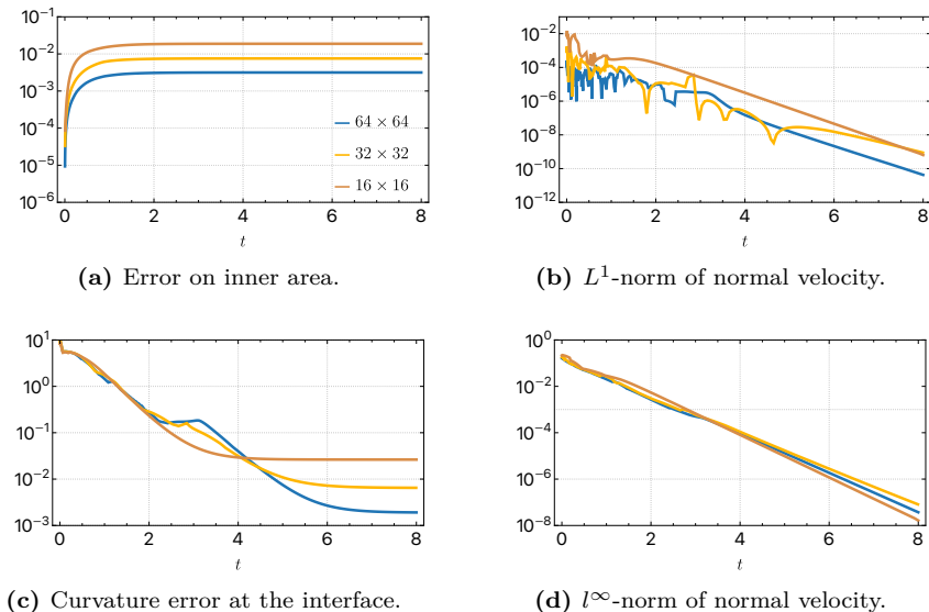
Figure 12: First verification test case: error indicators. The HHO polynomial order is k = 1 , and we employ q = 2 for the level-set approximation. The meshes are composed of 16 \times 16 (brown line), 32 \times 32 (yellow line) and 64 \times 64 (blue line) square cells. The interface discretization parameters are (l = 2, n = 0) . The number of fixed-point iterations is 100 for the case of the mesh composed of 16 \times 16 square cells, and 180 for the case of meshes composed of 32 \times 32 and 64 \times 64 square cells.
