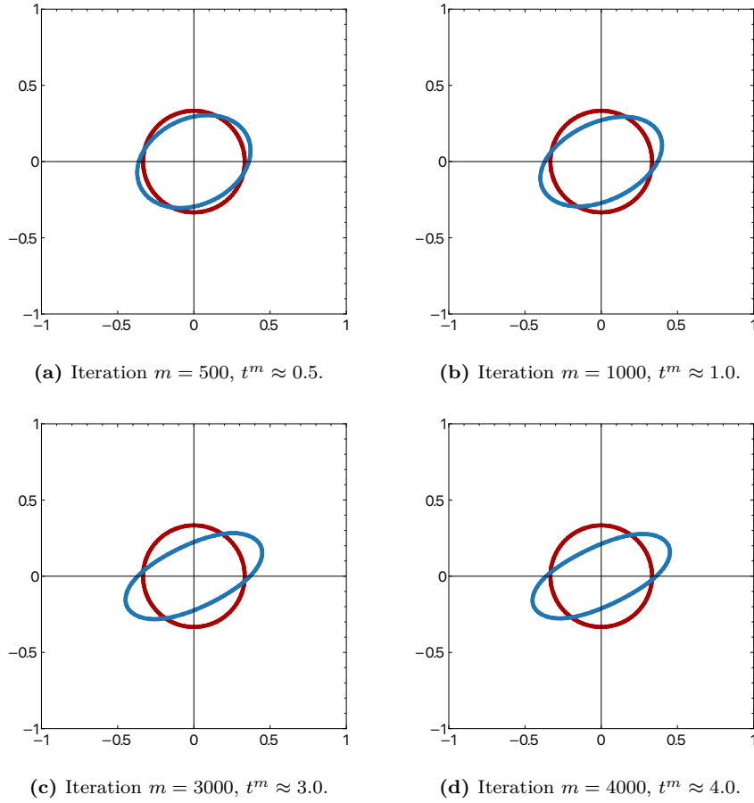
Figure 18: Interface evolution for the test case with unknown interface with Ca = 0.27 (i.e., \varepsilon = 0.26 , \gamma = 1 , \mu_2 = 1 , R_* = 1/3 ). In each panel, the red bullets represent the initial interface, and the blue ones the interface at iteration m of the fixed-point procedure. The HHO polynomial order is k = 1 , and we employ q = 2 for the level-set approximation. The mesh is composed of 128 \times 128 square cells. The interface discretization parameters are (l = 2, n = 0) .
