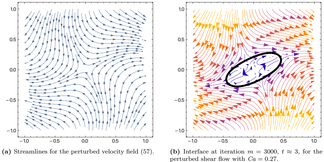
Figure 17: Streamlines for the test case with unknown interface. Figure 17.a illustrates the velocity field (57) without the interface (i.e., \gamma = 0 ), Figure 17.b includes the presence of the interface with Ca = 0.27 (i.e., \varepsilon = 0.26 , \gamma = 1 , \mu_2 = 1 , R_* = 1/3 ). The HHO polynomial order is k = 1 , and we employ q = 2 for the level-set approximation. The mesh is composed of 128 \times 128 square cells. The interface discretization parameters are (l = 2, n = 0) .
