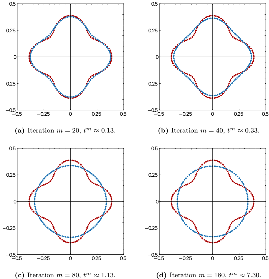
Figure 11: First verification test case. In each panel, the red bullets represent the initial interface, and the blue ones the interface at iteration m of the fixed-point procedure. The HHO polynomial order is k = 1 , and we employ q = 2 for the level-set approximation. The mesh is composed of 32 \times 32 square cells. The interface discretization parameters are (l = 2, n = 0) .
