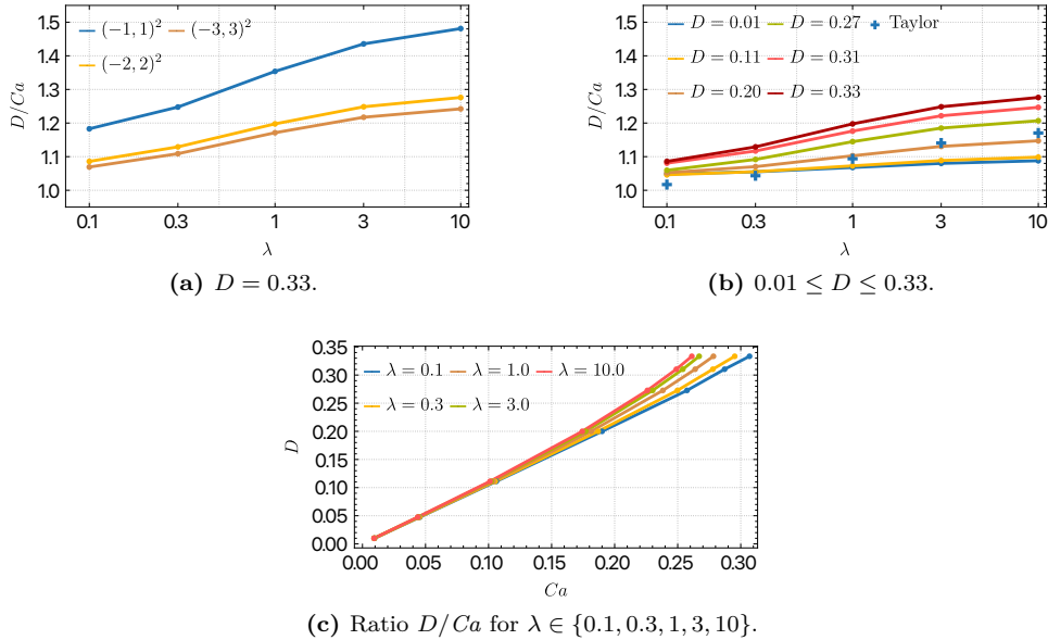
Figure 10: Figures 10.a and 10.b display the ratio D/Ca (Taylor deformation parameter over capillary number) as a function of the viscosity ratio \lambda . Figure 10.a: D = 0.33 and computational domains (-a, a)^2 with a \in \{1, 2, 3\} . Figure 10.b: D \in \{0.01, 0.11, 0.20, 0.27, 0.31, 0.33\} and computational domain (-2, 2)^2 ; the blue crosses refer to the estimate from [38] derived under the assumption of small deformations. Figure 10.c displays D as a function of Ca ; \lambda \in \{0.1, 0.3, 1, 3, 10\} and computational domain (-2, 2)^2 . We employ the unfitted HHO discretization with polynomial order k = 1 .
