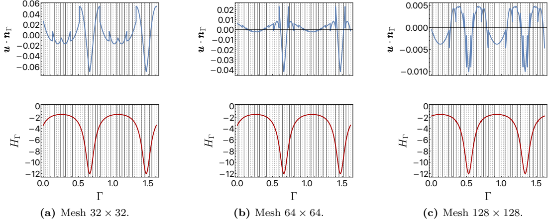
Figure 8: Normal velocity (blue, top row) and curvature (red, bottom row) along the interface. Shear-surface tension equilibrium with elliptic interface for D = 1/3 , \mu_1 = \mu_2 = 1 , Ca \in \{0.308, 0.274, 0.278\} using meshes composed of 32 \times 32 , 64 \times 64 and 128 \times 128 square cells, respectively (i.e., \varepsilon \in \{0.654, 0.581, 0.590\} , \gamma = 1 , R_1 = 1/6 and R_2 = 1/3 ) in the domain (-2, 2)^2 . We employ the unfitted HHO discretization with polynomial order k = 1 .
