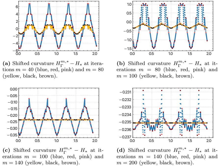
Figure 13: First verification test case. Shifted curvature H_{\Gamma}^{m,*} - H_* (see (53)) as a function of the curvilinear abscissa along the interface at iteration m \in \{40, 80, 100, 140, 200\} of the fixed-point procedure. For all the cut cells T \in \mathcal{T}^{T^m} , the blue (or yellow) bullets represent the values at the points inside T , the red (or black) bullets the values at the points on the boundary of T , and the pink (or brown) bullets the values at the points on the boundary of the agglomerated cells inside T . The HHO polynomial order is k = 1 , and we employ q = 2 for the level-set approximation. The mesh is composed of 32 \times 32 square cells. The interface discretization parameters are (l = 2, n = 0) .
