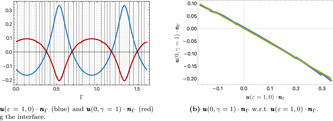
Figure 7: Figure 7.a: normal velocities along the interface; the dashed vertical lines in the background represent the intersections between the interface and the cell faces, whereas the solid lines represent the intersections between the interface and the erased inner faces of the agglomerated cells. Figure 7.b: \mathbf{u}(0, \gamma = 1) \cdot \mathbf{n}_\Gamma versus \mathbf{u}(\varepsilon = 1, 0) \cdot \mathbf{n}_\Gamma (blue bullets); the green line represents the linear regression curve with slope -m \approx 0.590 . Elliptic interface with D = 1/3 and \mu_1 = \mu_2 = 1 . The velocity fields \mathbf{u}(\varepsilon = 1, 0) and \mathbf{u}(0, \gamma = 1) are computed in the domain \Omega = (-2, 2)^2 discretized by a mesh composed of 128 \times 128 square cells. We employ the unfitted HHO discretization with polynomial order k = 1 .
