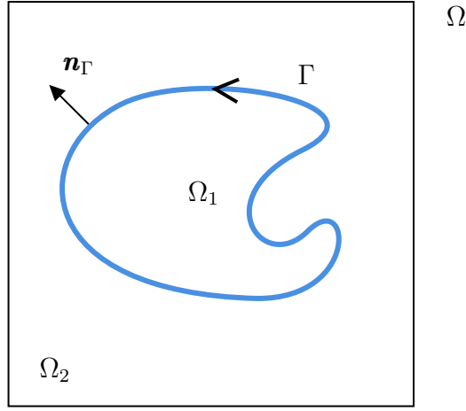
Figure 1: Computational domain \Omega , subdomains \Omega_i , i \in \{1, 2\} , interface \Gamma , and unit normal \mathbf{n}_\Gamma .
