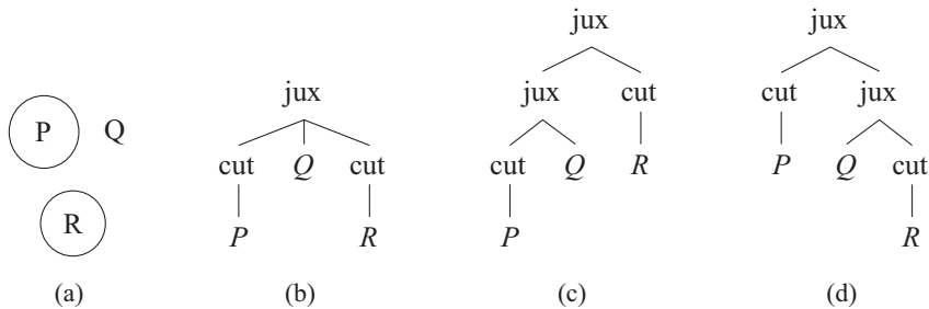
Figure 5. An AG with three possible parsing trees.
