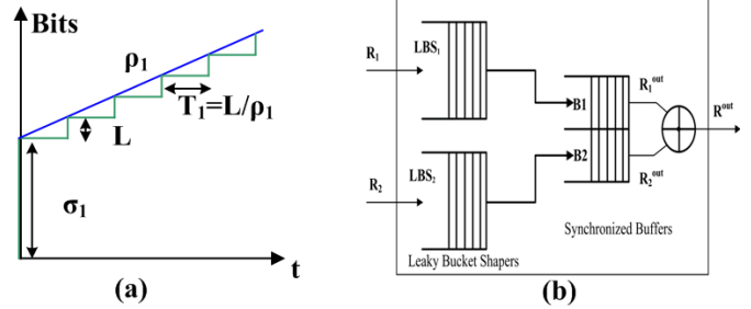
Figure 1: (a) staircase arrival curve. (b) coding node Architecture.
