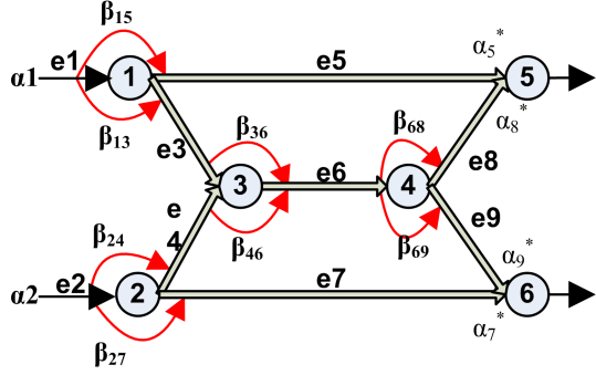
Figure 2: Simple delay-free, acyclic, directed network with two sources A and B generating the input flows R_1, R_2 with respective arrival curves \alpha_1 and \alpha_2 . The two sinks (or receiver nodes) are the nodes 5) and 6). The nodes 1), 2), 3) and 4) are the Coding Nodes . Each node offers a given service curve to their input flows toward their output flows.
