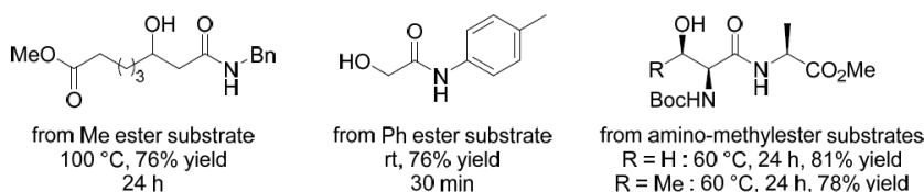
Scheme 25. Hydroxy-directed amidation of esters with Ta(OEt) 5 .
