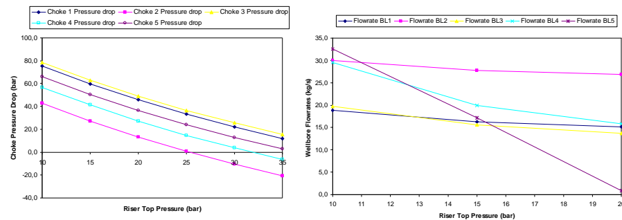
Figure 3.: Results from various riser top pressure specifications a. (left): Cases without recycle – FP strategy b. (right): Cases without recycle – PP strategy
