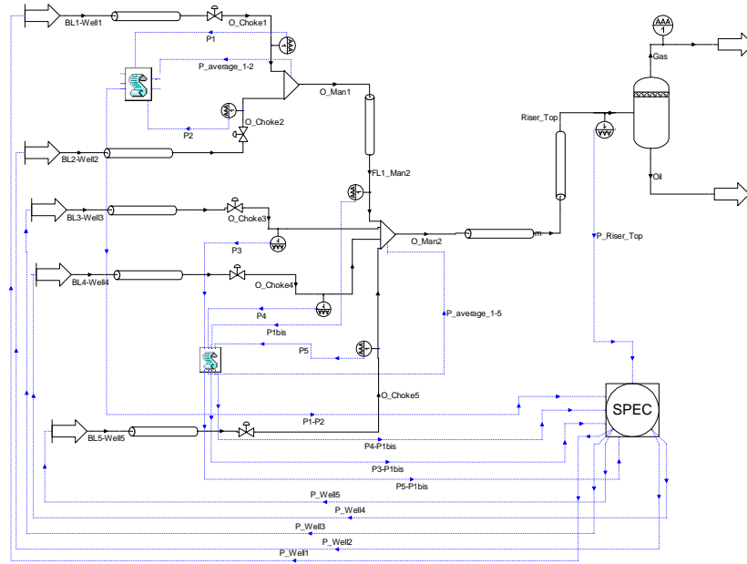
Figure 2. : Base Case Flowsheet
