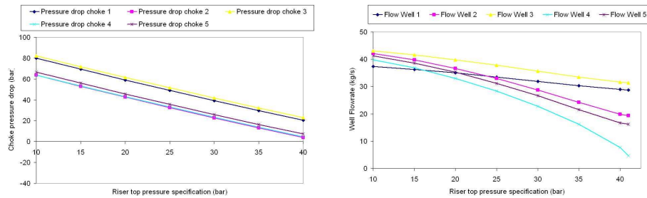
Figure 5.: INDISS-TINA results from various riser top pressure specifications a. (left): Cases without recycle – FP strategy b. (right): Cases without recycle – PP strategy
