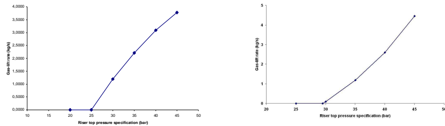
Figure 4. : Cases with recycle – FP strategy Results from various riser top pressure specifications a. (left) ProsimPlus™ results b. (right) INDISS-TINA results
