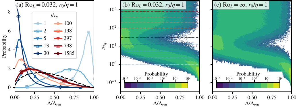
FIG. 10. Probability density function (PDF) of the tetrad shape parameter \Lambda . (a) PDF of \Lambda at different times under intense rotation ( Ro_L = 0.032 , run 4) for tetrads of initial scale r_0 = \eta . Dashed black line: PDF of \Lambda in the isotropic diffusive regime obtained from Monte Carlo simulations. (b) Alternative representation of the PDF of \Lambda at different times, for the same case shown in (a). Each horizontal cut of the contour plot represents the PDF at a given time. Dash-dotted horizontal lines correspond to the different times plotted in (a). (c) Similar to (b) but for the nonrotating run (run 1).
