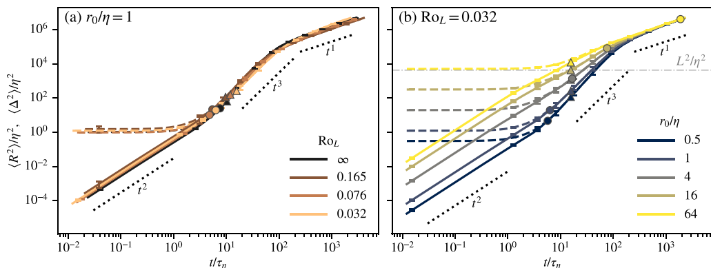
FIG. 5. Mean-squared separation between Lagrangian pairs. Dashed lines, mean-squared gyration radius \langle R^2 \rangle [Eq. (2)]; solid lines, mean-squared change of gyration radius \langle \Delta^2 \rangle [Eq. (3)]. Distances are normalized by the Kolmogorov scale \eta . (a) Pairs of initial scale r_0 = \eta and different rotation rates. (b) Pairs of different initial scales r_0 under intense rotation ( Ro_L = 0.032 , run 4). Markers represent the ballistic timescale t_0 = \langle (\delta \mathbf{v}_0)^2 \rangle / |\langle \delta \mathbf{v}_0 \cdot \delta \mathbf{a}_0 \rangle| (circles) and the vertical Lagrangian integral time scale T_L^z (triangles) for the different cases. Note that, for particle pairs, the gyration radius R is directly related to the pair separation vector \delta \mathbf{X} as R(t)^2 = |\delta \mathbf{X}(t)|^2 / 2 . Equivalently, \Delta(t)^2 = |\delta \mathbf{X}(t) - \delta \mathbf{X}(0)|^2 / 2 . In (b), the horizontal dash-dotted line corresponds to L^2/\eta^2 , where L is the Eulerian integral length scale. Error bars are obtained after splitting each dataset onto four disjoint sub-data-sets. The size of the error bars corresponds to the standard deviation of the statistics computed from each separate sub-data-set. Throughout our results, error bars are rather small, especially when plotted in logarithmic scale. In the following, for ease of readability, error bars are not shown for quantities plotted in logarithmic scale.
