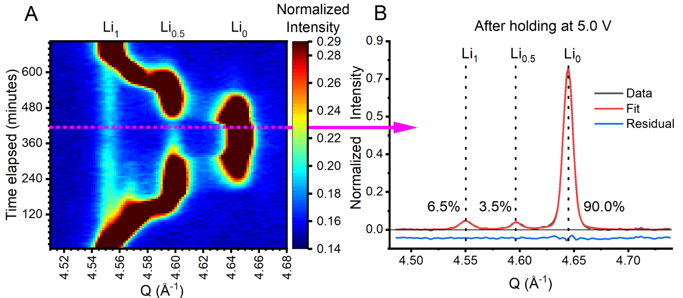
Figure 2: Waterfall plot of the diffraction intensities of the Li 1 , Li 0.5 , and Li 0 peaks for the LMNO 531 reflection, with contrast adjusted to show the trace quantities of the inactive phases. (A) Powder diffraction after 1 hour hold at 5.0 V (B, extracted from magenta line in A). Each of the Li 1 , Li 0.5 , and Li 1 phases were background subtracted, fit with pseudo-Voigt lineshapes, and integrated.
