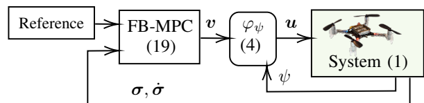
Fig. 1. Flatness-based MPC control scheme.
