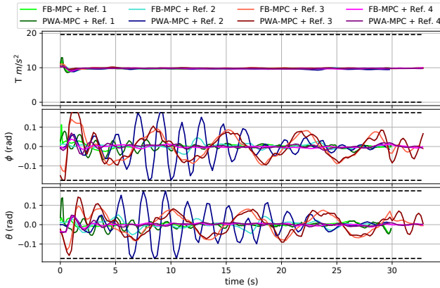
Fig. 8. Input signals with their constraints (black dashed line).
