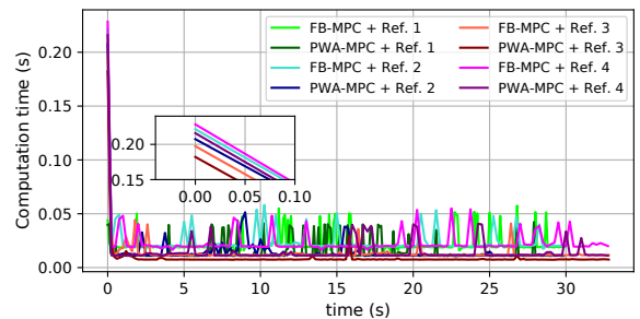
Fig. 6. Computation time used for different references.
