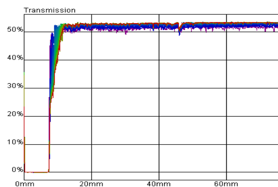
Figure 6b: Diffuse transmittance of Klebosol 30R50 3 % wt.
