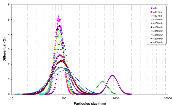
Figure 14a: Differential particle size distributions during the aggregation of Klebsol 30R50 (wt. 1%) by sodium chloride solution (0,8M) for 0^+ < t < 300 min.
