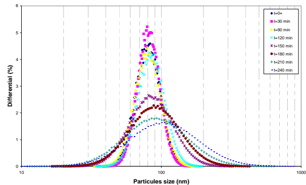
Figure 14b: Differential particle size distributions during the aggregation of Klebsol 30R50 (wt. 1%) by sodium chloride solution (0,8M) for 0^+ < t < 240 min.
