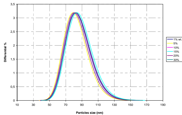
Figure 11: Particles size distributions of different Klebsol 30R50 suspensions measured with the Ultrasizer
