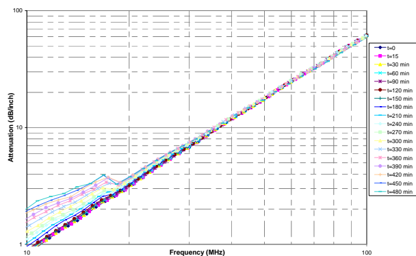
Figure 12: Attenuation spectra of Klebsol 30R50 during the aggregation process
