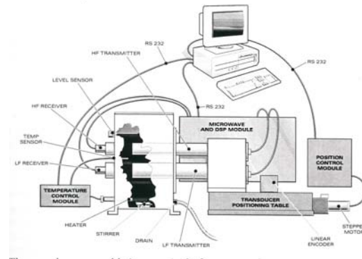
Figure 4: Experimental set-up
