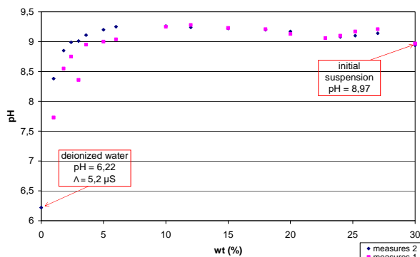
Figure 5 : Evolution of pH versus solid content of Klebosol 30R50
