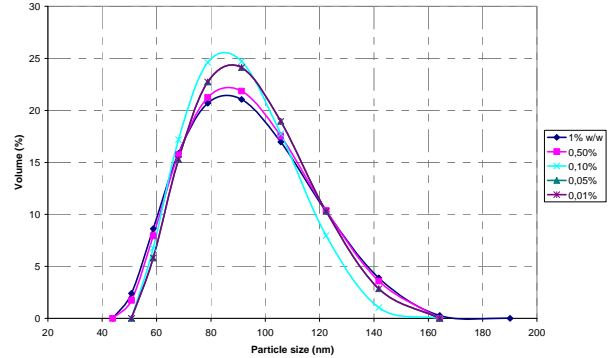
Figure 8: Particle size distributions of different Klebosol 30R50 suspensions measured with the Zétasizer NanoS
