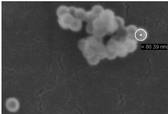
Figure 1: SEM photography of Klebosol 30R50 (x 50000)
