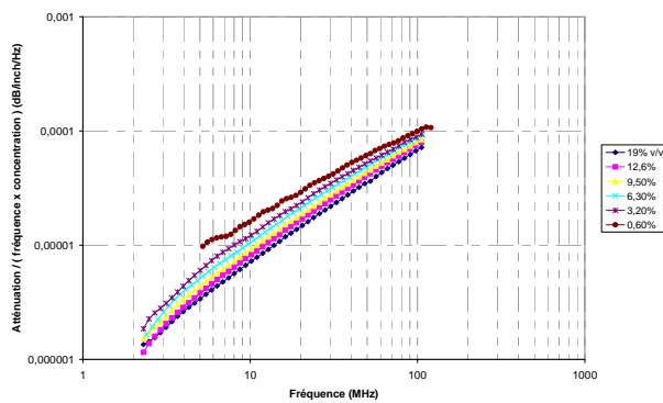
Figure 10: Excess attenuation spectra of Klebsol 30R50 normalized by the frequency and the volume concentration for different concentrations
