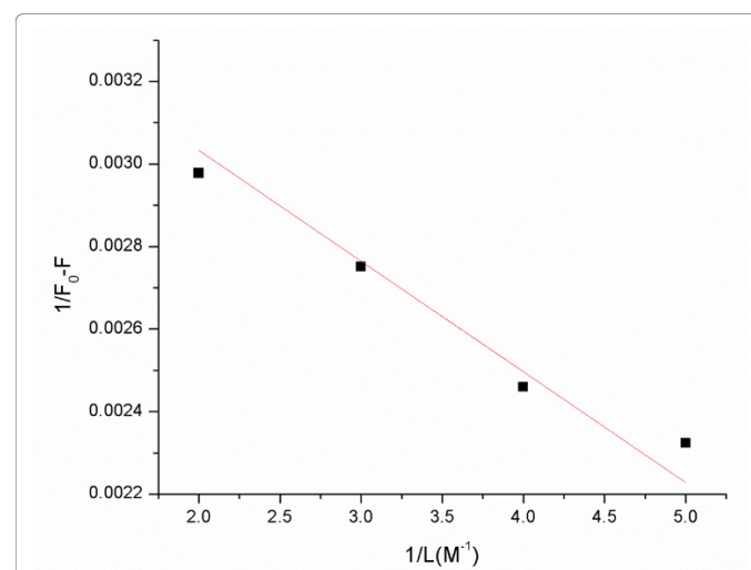
Figure 10: The plot of 1/(F_0 - F) vs. (1/L) \times 10^4 for gold nanoparticles 60 nm-BSA complexes.
