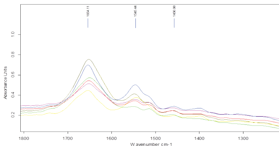
Figure 13: The spectrum of Gold nanoparticles 60 nm-BSA complexes with different percentage of gold nanoparticles.
