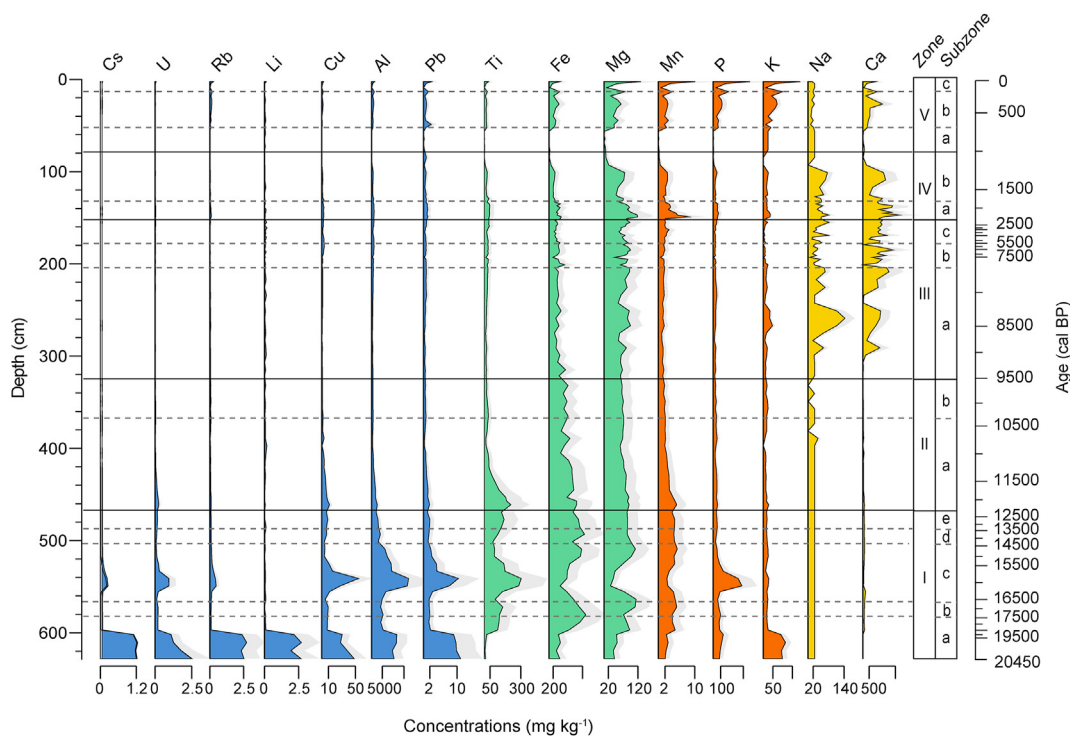
Fig. 9. ICP-MS record of CEN-17.4 showing selected element concentrations ( mg\ kg^{-1} ), coloured by dominance in each pollen assemblage zone (determined via indicator analysis), against depth (cm) and age (cal BP).
