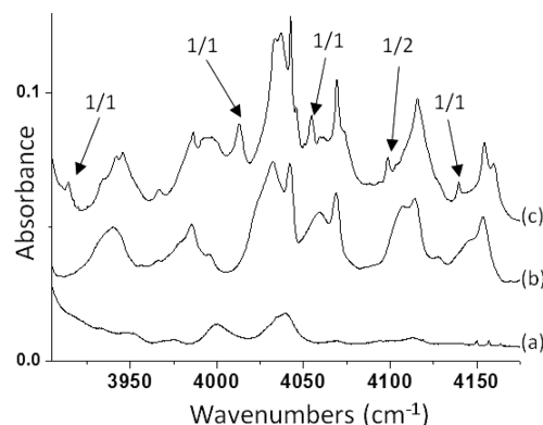
Figure 5. Neon matrix spectra after deposition at 3.5 K recorded in the 3900–4200 cm -1 region of ν(OH) + ν inter combinations of small H 2 O and DAC–H 2 O clusters for different dilutions of the ternary mixture DAC/H 2 O/Ne: (a) 6/0/1000, (b) 0/2/1000, (c) 3/3/1000.
