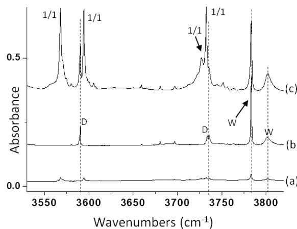
Figure 3. Neon matrix spectra after deposition at 3.5 K recorded in the OH stretching region of \text{H}_2\text{O} monomer, \text{H}_2\text{O} and 1/1 dimers for different dilutions of the ternary mixture DAC/ \text{H}_2\text{O}/\text{Ne} : (a) 2/0/1000, (b) 0/1/16000, and (c) 1/0.025/1000. The notation W stands for \text{H}_2\text{O} monomer and D for water dimer.
