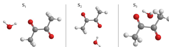
Figure 1. Three isomers for the 1/1 complex optimized at the MP2/AVTZ level of theory.
