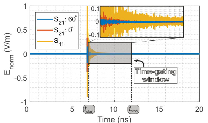
Fig. 15: Temporal domain filtered signals in mono-static and bistatic configurations considering the presence of an object. The time start ( t_{start} = 6.82 ns) and time stop t_{stop} = 12 ns of the time-gating window for the analyzed signals.
