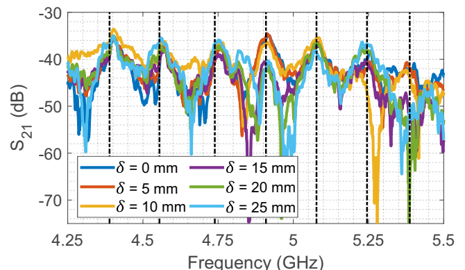
Fig. 23: Misalignment study with a metal plate: |S_{21}(\beta = 60^\circ)| measurements for different \delta values.
