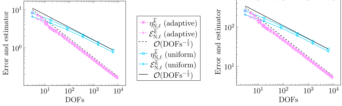
Figure 7: [Exponential nonlinearity (6.5), singular solution (6.6), L-shaped domain, uniform vs adaptive mesh refinement] Convergence of \mathcal{E}_{N,\ell}^k and \eta_{N,\ell}^k with respect to the number of degrees of freedom for uniform and adaptive mesh refinement for a_c/a_m equal to 10^3 (left) and 10^6 (right).
