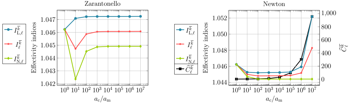
Figure 3: [Exponential nonlinearity (6.5), smooth solution (6.3), unit square domain, 3969 DOFs] Effectivity indices from (6.1) and the computable constant \hat{C}_\ell^k from (5.11).
