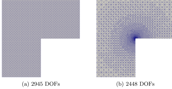
Figure 5: Uniformly (left) and adaptively (right) refined meshes for the L-shaped domain with the singular solution (6.6). The adaptive mesh corresponds to \ell = 28 in Algorithm 6.3.
