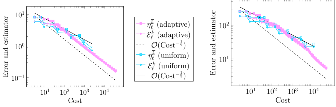
Figure 10: [Exponential nonlinearity (6.5), singular solution (6.6), L-shaped domain, uniform vs adaptive mesh refinement] Convergence of \mathcal{E}_\ell^k and \eta_\ell^k with respect to cost for uniform and adaptive mesh refinement for a_c/a_m equal to 10^3 (left) and 10^6 (right).
