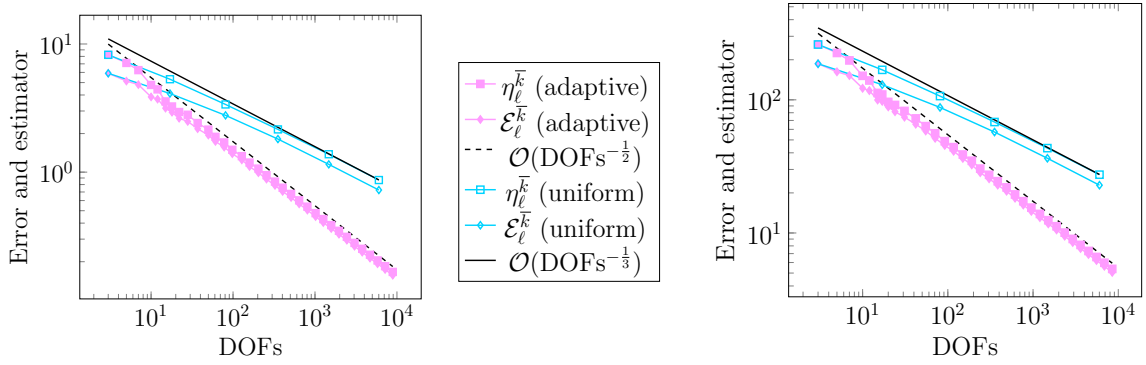
Figure 8: [Exponential nonlinearity (6.5), singular solution (6.6), L-shaped domain, uniform vs adaptive mesh refinement] Convergence of \mathcal{E}_\ell^k and \eta_\ell^k with respect to the number of degrees of freedom for uniform and adaptive mesh refinement for a_c/a_m equal to 10^3 (left) and 10^6 (right).
