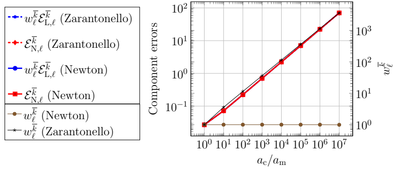
Figure 4: [Exponential nonlinearity (6.5), smooth solution (6.3), unit square domain, 3969 DOFs] Components \mathcal{E}_{N,\ell}^k and w_\ell^k \mathcal{E}_{L,\ell}^k from (5.5) together with the weight w_\ell^k from (5.4). The four curves of w_\ell^k \mathcal{E}_{L,\ell}^k and \mathcal{E}_{N,\ell}^k essentially coincide.
