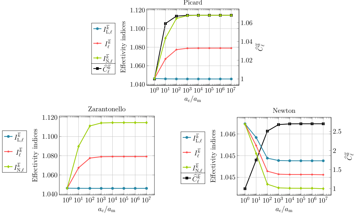
Figure 2: [Mean curvature nonlinearity (6.4), smooth solution (6.3), unit square domain, 3969 DOFs] Effectivity indices from (6.1) and the computable constant \hat{C}_\ell^k from (5.11).
