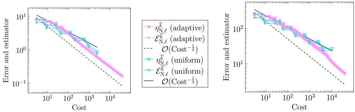
Figure 9: [Exponential nonlinearity (6.5), singular solution (6.6), L-shaped domain, uniform vs adaptive mesh refinement] Convergence of \mathcal{E}_{N,\ell}^k and \eta_{N,\ell}^k with respect to cost for uniform and adaptive mesh refinement for a_c/a_m equal to 10^3 (left) and 10^6 (right).
