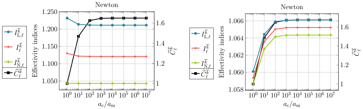
Figure 6: [Exponential nonlinearity (6.5), singular solution (6.6), L-shaped domain] Effectivity indices from (6.1) and the computable constant \hat{C}_\ell^k from (5.11), for the uniform mesh (left) and the adaptive mesh (right) shown in Figure 5.
