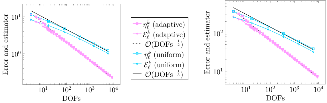
Figure 8: [Exponential nonlinearity (6.5), singular solution (6.6), L-shaped domain, uniform vs adaptive mesh refinement] Convergence rates of \mathcal{E}_\ell^k and \eta_\ell^k for uniform and adaptive mesh refinement for a_c/a_m equal to 10^3 (left) and 10^6 (right).
