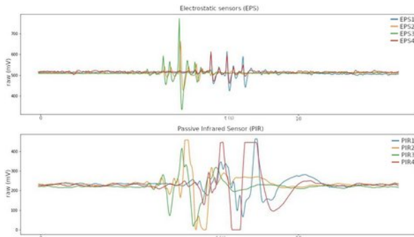
Figure 5: Graph of data acquired by PIR and EPS for a medium walking speed.
