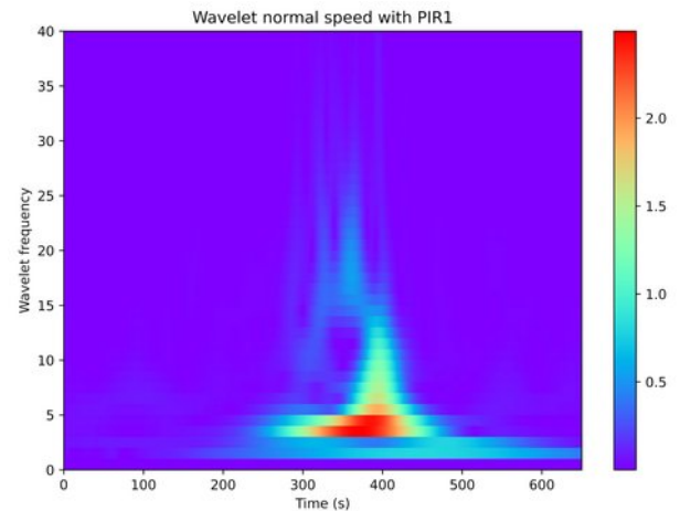
Figure 7: Morlet wavelet transform of PIR signal for a walking person.
