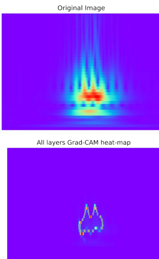
Figure 9: A wavelet transform as one of the Grad-CAM input and the corresponding heatmap for the trained 2-Layer NN
