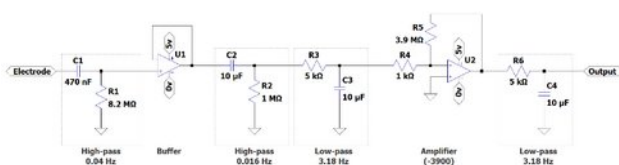
Figure 2: Electrical Diagram of the EPS
