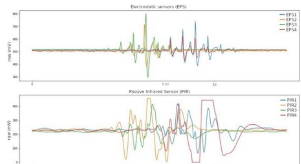
Figure 4: Graph of data acquired by PIR and EPS for a slow walking speed.
