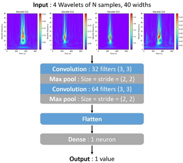
Figure 7: Parameters of the CNN model giving the lowest reproducible uncertainty.
