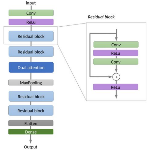
Figure 8: ResNet architecture giving the lowest uncertainty.
