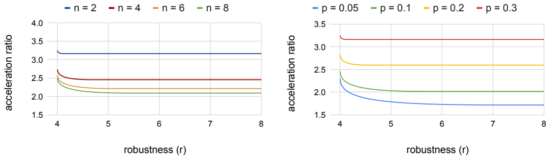
(a) The value of p is fixed to p = 0.1 . (b) The number of queries is fixed to n = 10
