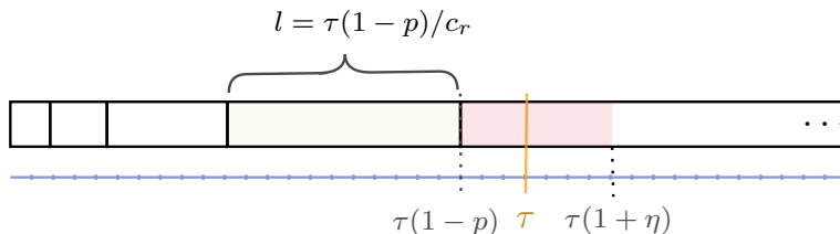
Figure 3: An illustration of Lemma 4. Assuming negative error at most p , the interruption occurs no earlier than \tau(1-p) , and no later than \tau(1+\eta) for positive error \eta . In the former case, in particular, a contract of length l = \frac{\tau(1-p)}{c_r} is guaranteed to be completed by the interruption time.
