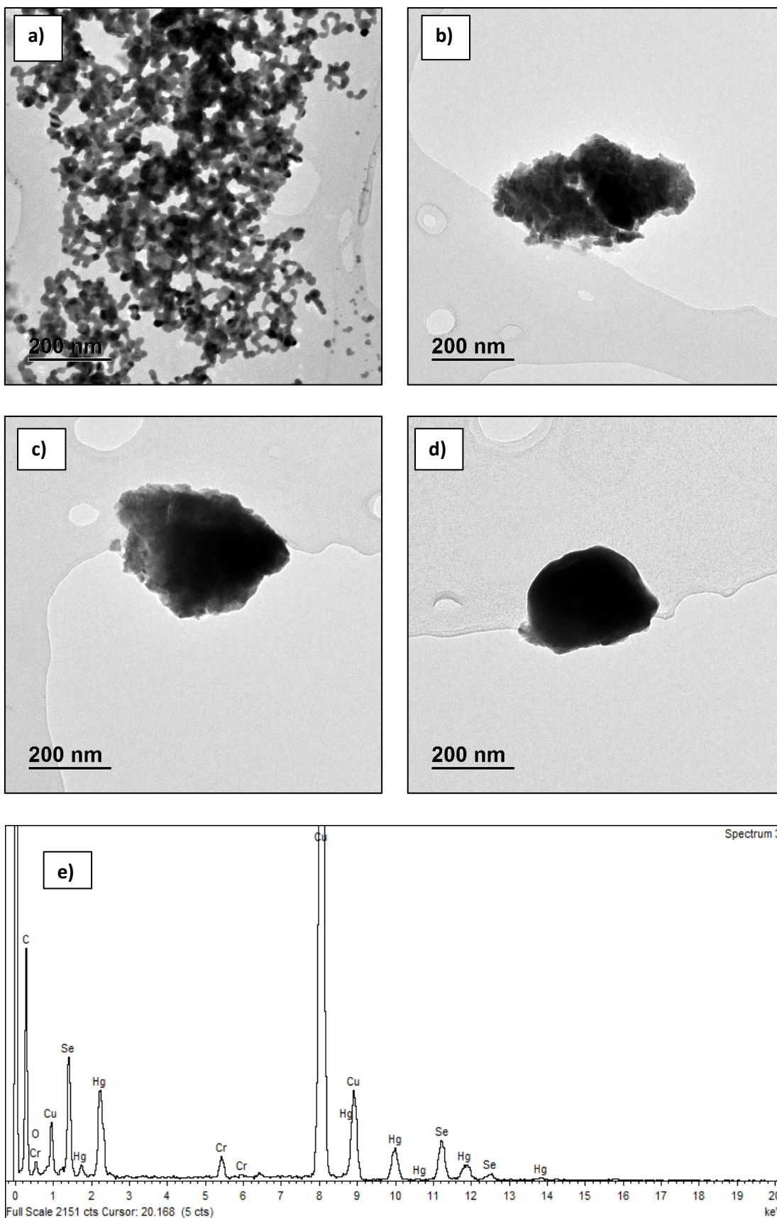
Figure 1. TEM images of the HgSe NPs standard dispersed in: (a) Milli-Q water, (b) \phi = 50\% formic acid, (c) 2 \text{ mg mL}^{-1} protease K in 50 \text{ mmol L}^{-1} ammonium bicarbonate buffer (pH 7.4) (d)
