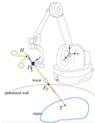
Fig. 3 Representation of the robotic arm and its kinematics.
