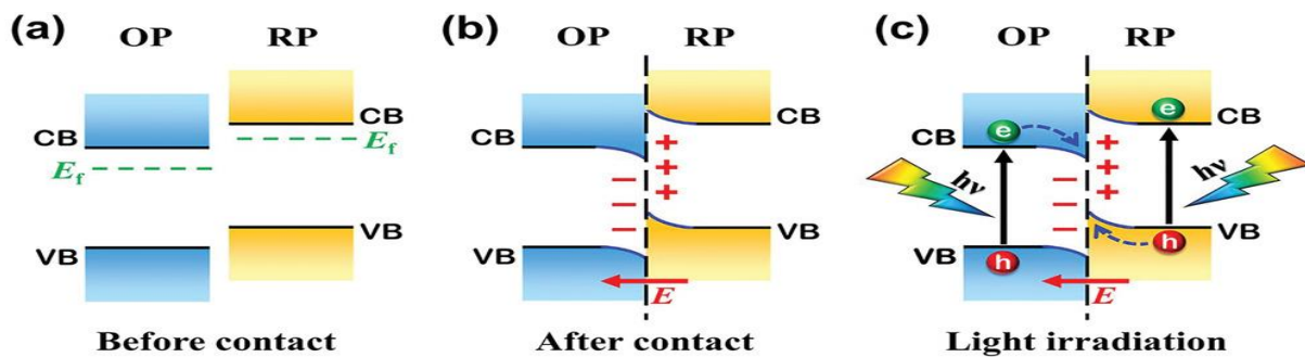
707 708 Figure 8: Mechanism of charge transfer in S-scheme heterojunction. Adapted with the 709 permission from ref. [125]. Copyright (2022) Wiley Online Library.
