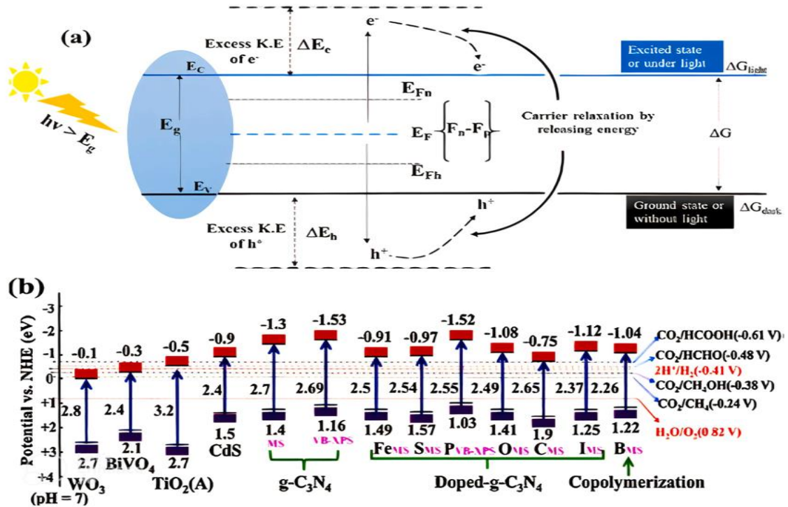
256 Figure 2: \Delta G and semiconductor thermodynamics with and without illumination (a); 257 semiconductor band potential and their applicability for forming value-added-products 258 (b). Adapted with permission from [26]. Copyright (2018) Elsevier
