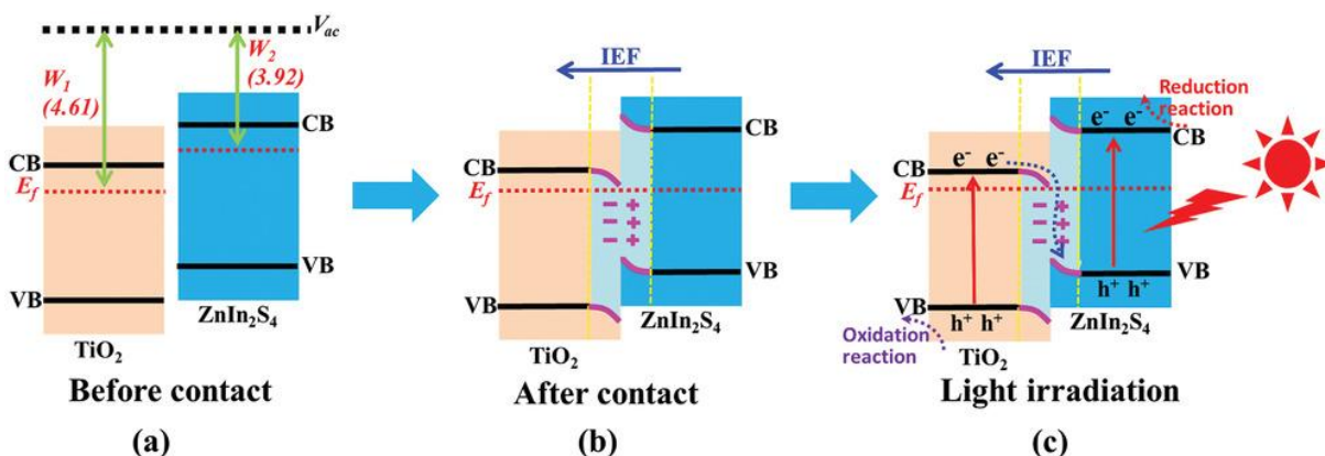
714 715 Figure 11: Charge transfer mechanism of hierarchical S-scheme TiO 2 @ZnIn 2 S 4 716 heterojunction. Adapted with the permission from ref. [122]. Copyright (2021) Wiley 717 Online Library
