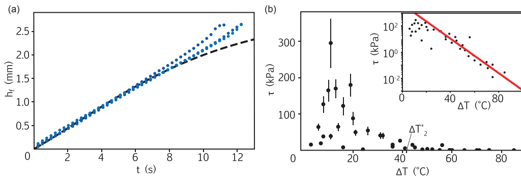
FIG. 5. (a) Experimental front h_f(t) for \Delta T = (50.2, 59.5, 79.1) C (blue points) and theoretical front for a spherical drop with T_s = -41 C (dashed line). (b) Adhesion of a water droplet to the copper substrate \tau as a function of \Delta T . Log-linear plot in the inset showing an exponential decrease.
