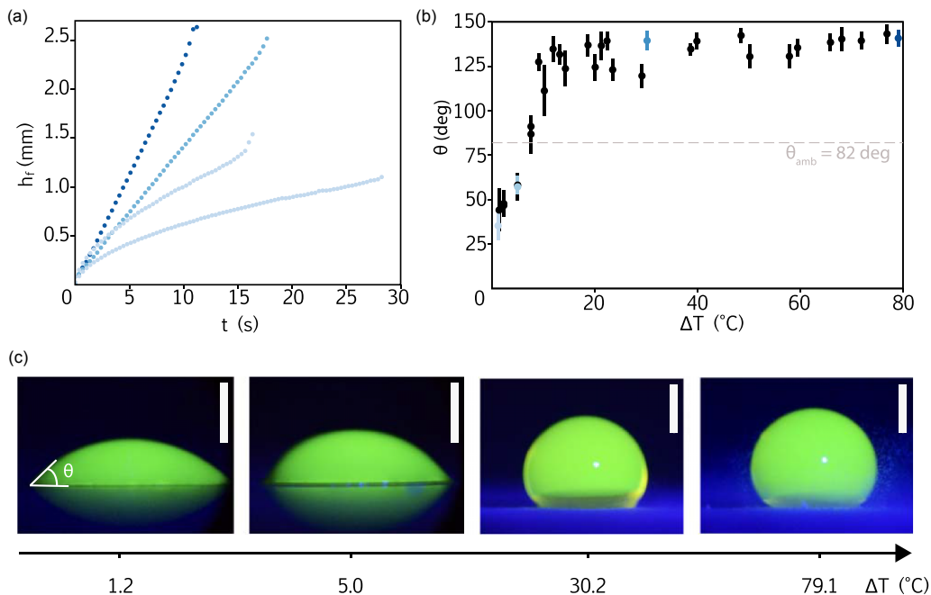
FIG. 2. (a) Front height h_f (mm) vs time t (s) for different temperatures (from lighter blue to darker blue) ( T_s, V ) = [(-1.2, 7), (-5.0, 7), (-30.2, 13), (-79.1, 13)] (C, \mu L). (b) The contact angle \theta vs \Delta T . Blue points correspond to the experiments presented in (a). The dashed gray line represents the contact angle at ambient temperature. (c) Snapshots of drops at different substrate temperatures and volumes ( T_s, V ) = [(-1.2, 7), (-5.0, 7), (-30.2, 13), (-79.1, 13)] (C, \mu L) corresponding to freezing fronts presented in (a). The scale bar represents 1 mm.
