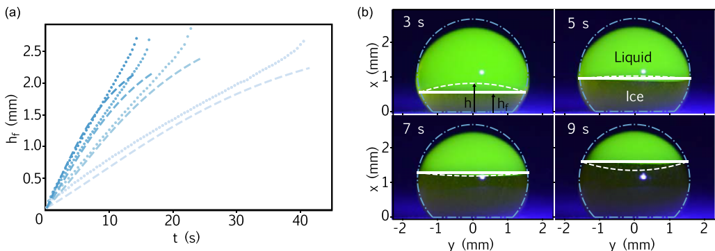
FIG. 4. (a) Theoretical fronts (dashed lines) and experimental fronts (dots) h_f(t) for \Delta T = 11.9, 23.5, 29.2, 38.7 C (from light to dark blue). (b) Overlay of theoretical drop profile (blue line) and freezing front at the edges (white line) and at the center (dotted white line) of a spherical drop for different times at \Delta T = 38.7 C. The experimental front corresponds to the interface between the liquid part which fluoresces green and the dark solid part which no longer contains fluorescein.
