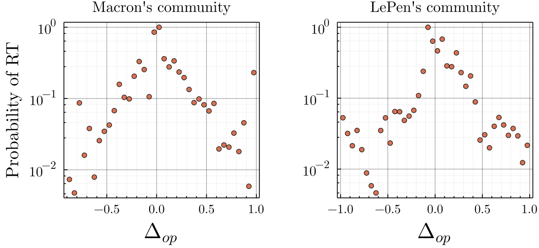
FIGURE 2 – Estimated probability for a user, in the ideological neighborhood of Emmanuel Macron or Marine Le Pen, to retweet a read message according to the different of opinion with its author, \Delta_{op} = o_{reader} - o_{sender} , considering periodic boundary conditions. We renormalize such that a perfectly aligned message is retweeted with certainty.
