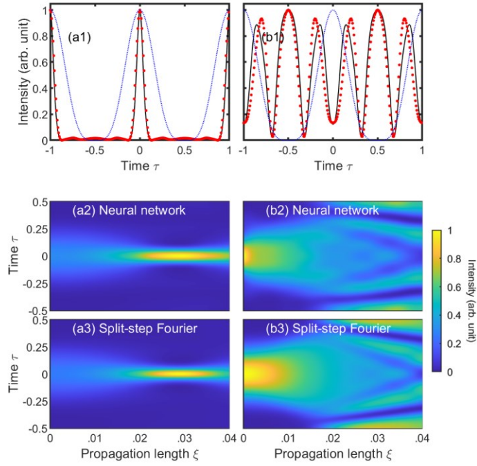
Figure 10: Temporal reshaping of an initially sinusoidal signal with A = 3 dB and N = 6 upon nonlinear propagation in the fibre. (a) Temporal narrowing in the anomalous dispersion regime and (b) formation of undular bores at normal dispersion. Panels 1 show the temporal intensity profiles at the point of maximum compression and after a propagation length of \xi = 0.04 , respectively. The predictions from the NN (red circles) are compared with the results of NLSE simulations (black curves). Also shown is the initial signal (blue curves). The waveforms are normalised to the same peak power. Panels 2 and 3 show the longitudinal evolutions of the temporal intensity profiles as obtained from the NN and NLSE simulations, respectively.
