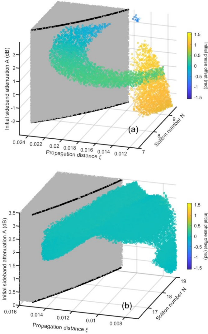
Figure 7: Regions in the space of input parameters (A, \varphi, \xi, N) that enable the formation of high-flatness combs starting from a three-frequency component initial condition. The results obtained for propagation in the anomalous and normal dispersion regimes of the fibre are shown in subplots (a) and (b), respectively. The data visualisation is restricted to the parameter volume where solutions are found, and the grey region represents volume that is unexplored.
