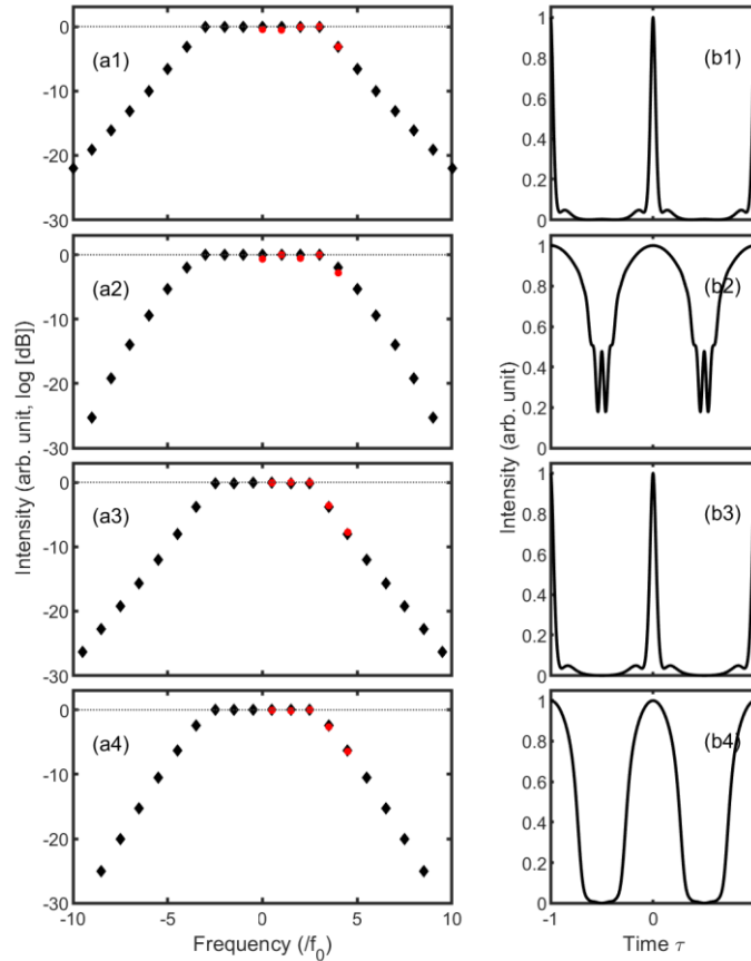
Figure 6: Generation of combs with six (panels 1, 2) and seven (panels 3, 4) spectral lines through nonlinear fibre propagation of three- and four-frequency component initial conditions, respectively. The results obtained in the anomalous and normal dispersion regimes of the fibre are shown in panels 1, 3, and 2, 4, respectively. (a) The optical spectra predicted by the NN (red circles) are compared with those obtained from NLSE simulations (black diamonds). (b) Corresponding temporal intensity profiles obtained from NLSE simulations.
