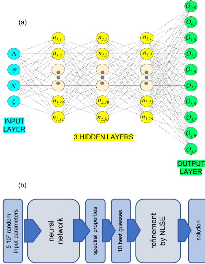
Figure 2: (a) NN architecture deployed. (b) Principle of searching for the optimum solution.
