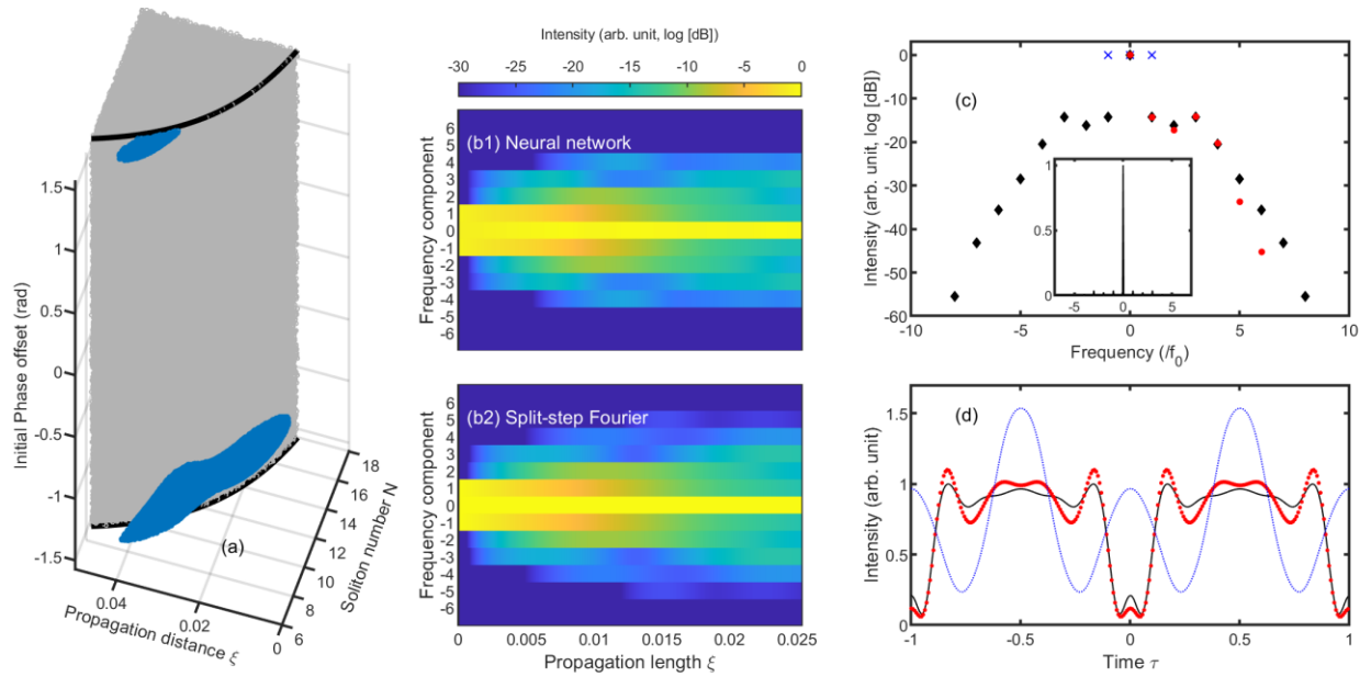
Figure 9: Spectral narrowing process. (a) Regions in the space of input parameters (\varphi, \xi, N) that enable focusing of more than 80% of the initial energy into the central frequency component, for an initial wave made of three initial spectral lines of equal amplitude and evolving in the normal dispersion regime of the fibre. (b) Longitudinal evolution of the optical spectrum obtained from the NN (panel 1) and NLSE simulations (panel 2). (c) Compressed optical spectrum plotted on a logarithmic scale. The predictions from the NN (red circles) are compared with the results of NLSE simulations (black diamonds). Also shown is the initial condition (blue crosses). The inset shows the compressed spectrum on a linear scale. (d) Corresponding temporal intensity profiles. The NN predictions, the results of NLSE simulations and the initial condition are plotted with red circles, a black curve, and a blue dotted curve, respectively. The waveforms are normalised to the same average power.
