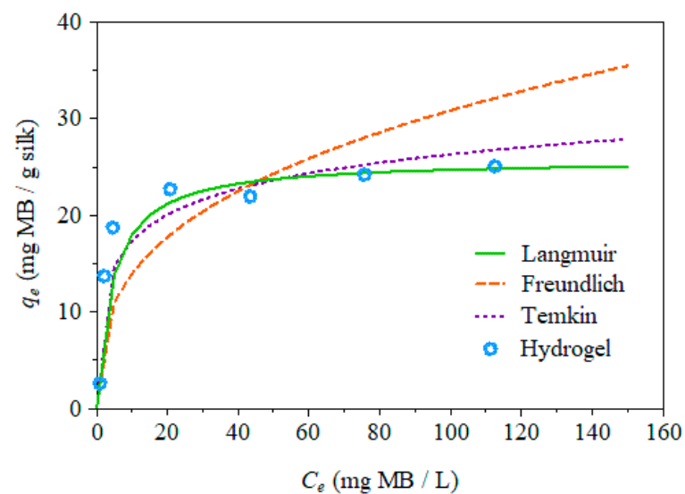
Figure 4. Methylene blue adsorption by SF hydrogels fitted to the Langmuir and Freundlich adsorption models. Best fit is found with the Langmuir model.
