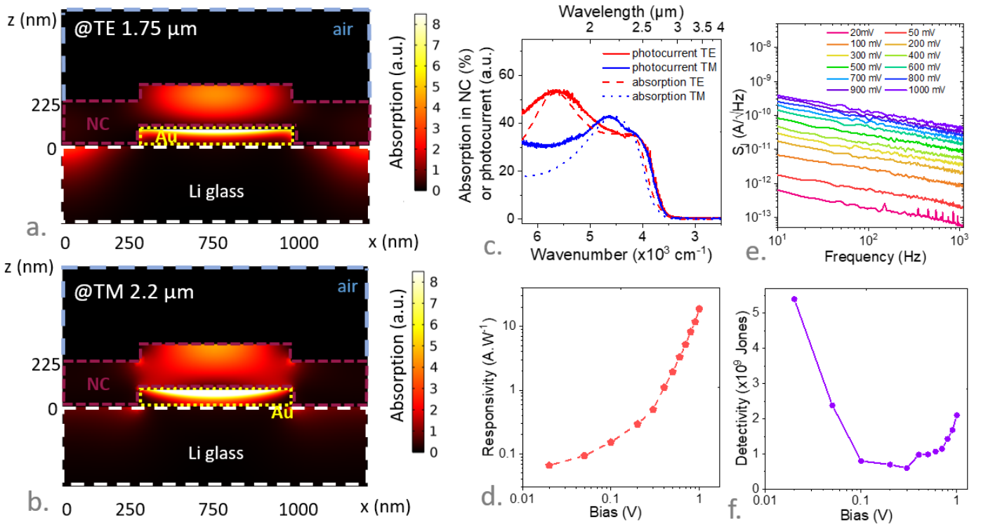
Figure 4 a. (resp b.) Simulated absorption map at the resonance of the TE @1.75 \mu\text{m} (resp TM at 2.2 \mu\text{m} ) polarization. c. Simulated absorption (dashed lines) and experimental photocurrent (solid lines) spectra within the NCs film (i.e., excluding losses in contact) for TE, TM polarization. d. Responsivity measured at 180 K for a signal at 1 kHz as a function of applied bias for the device with light resonators under broadband radiation resulting from a blackbody at 980°C. e. Noise current spectral density as a function of signal frequency measured under various applied biases. f. Specific detectivity measured at 180 K (for a signal at 1 kHz) as a function of applied bias for the device with light resonators.
